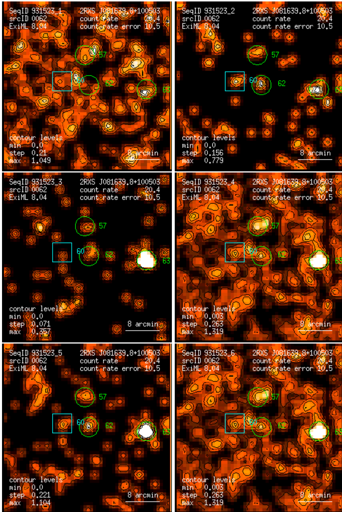
Figure 62: RASS 931523: detection 0062: band rate images, Gaussian filter: (1) PSPC channels 11 – 41, (2) 52 – 90, (3) 91 – 201, (4) 11 – 235, (5) 52 – 201, (6) 11 – 201. Broad band rates in counts/ks. Band rate contour levels in counts/ks/arcmin 2 .
