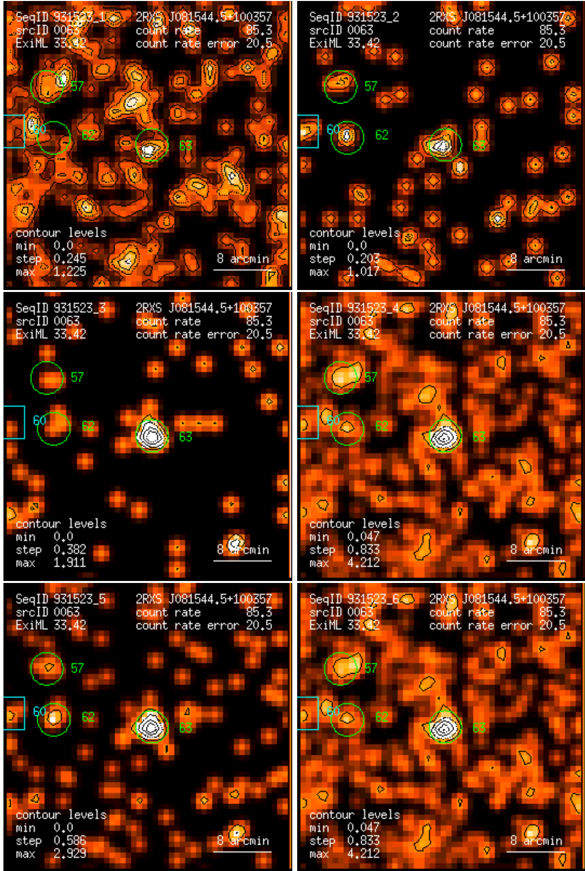
Figure 63: RASS 931523: detection 0063: band rate images, Gaussian filter: (1) PSPC channels 11 – 41, (2) 52 – 90, (3) 91 – 201, (4) 11 – 235, (5) 52 – 201, (6) 11 – 201. Broad band rates in counts/ks. Band rate contour levels in counts/ks/arcmin 2 .
