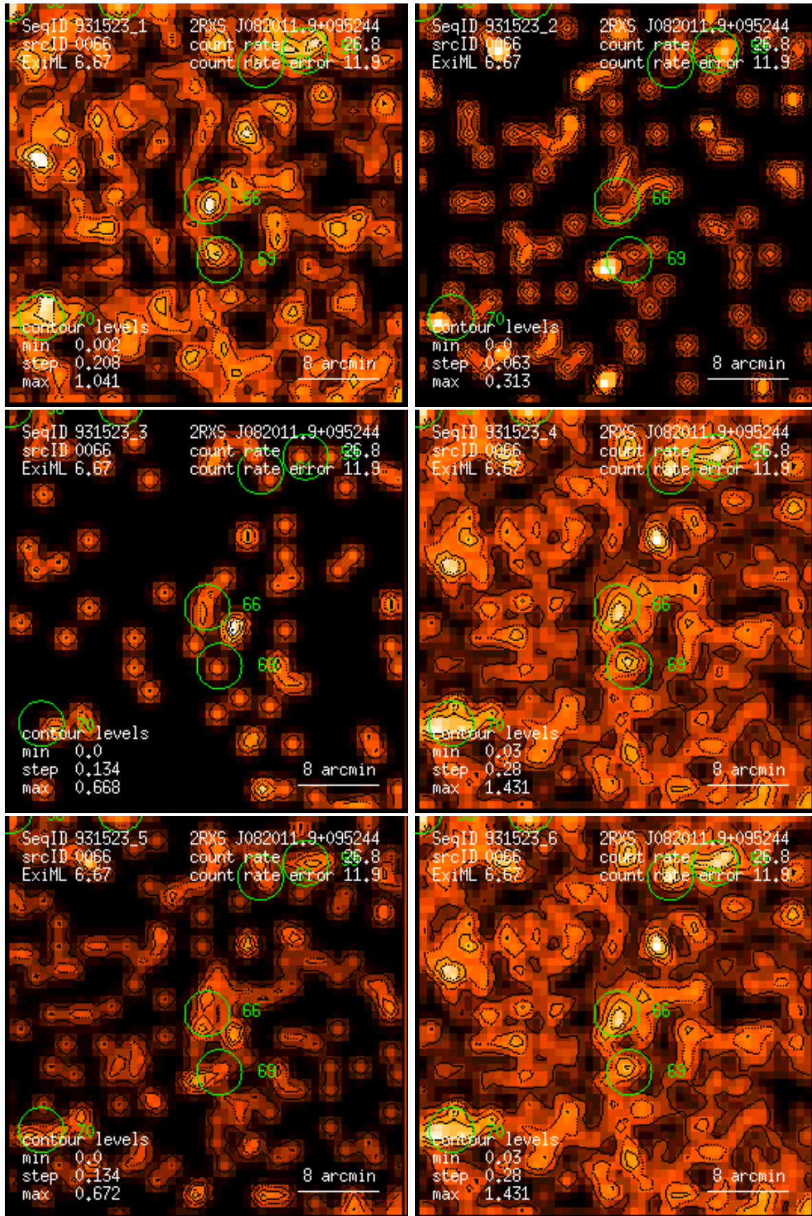
Figure 66: RASS 931523: detection 0066: band rate images, Gaussian filter: (1) PSPC channels 11 – 41, (2) 52 – 90, (3) 91 – 201, (4) 11 – 235, (5) 52 – 201, (6) 11 – 201. Broad band rates in counts/ks. Band rate contour levels in counts/ks/arcmin 2 .
