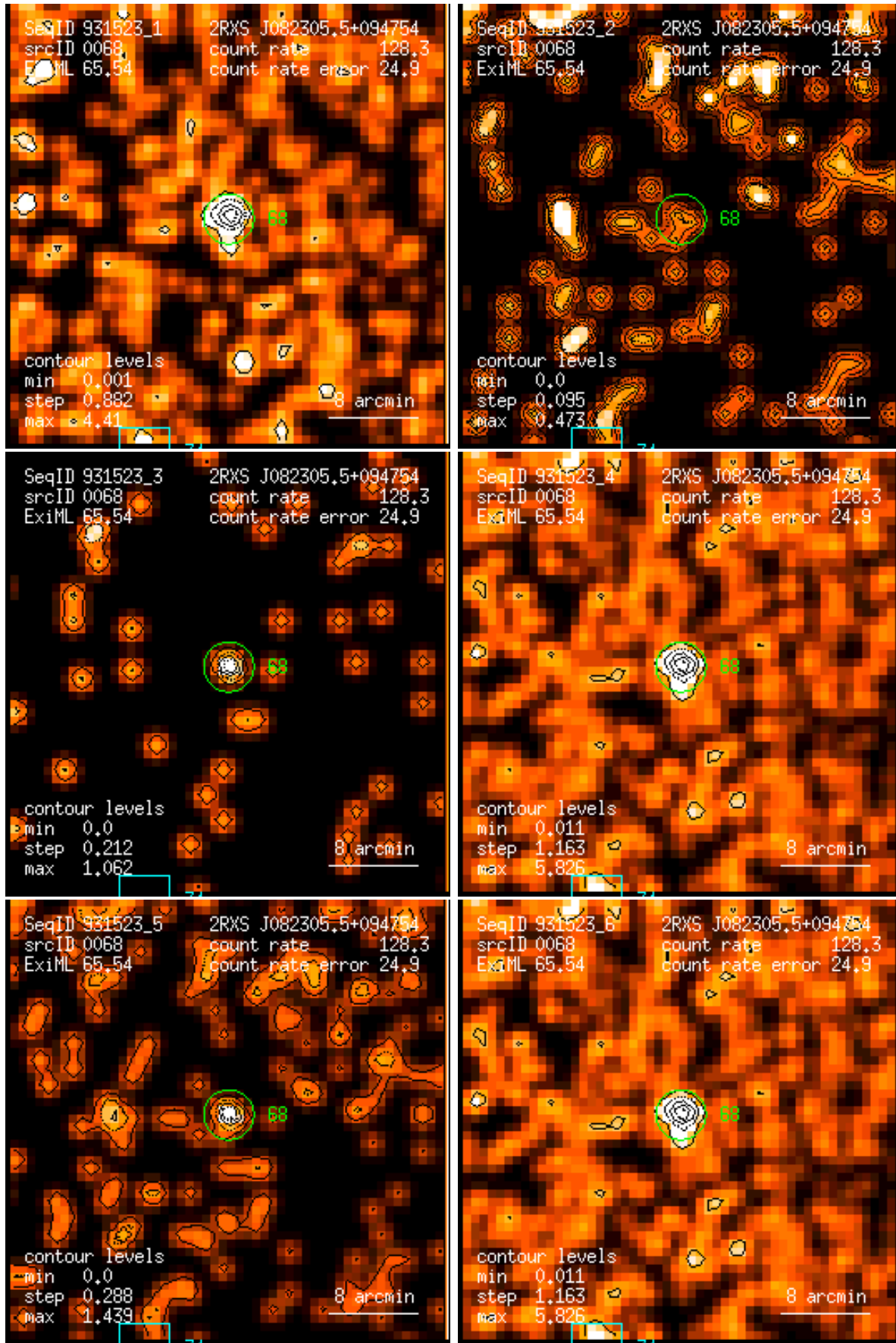
Figure 68: RASS 931523: detection 0068: band rate images, Gaussian filter: (1) PSPC channels 11 – 41, (2) 52 – 90, (3) 91 – 201, (4) 11 – 235, (5) 52 – 201, (6) 11 – 201. Broad band rates in counts/ks. Band rate contour levels in counts/ks/arcmin 2 .
