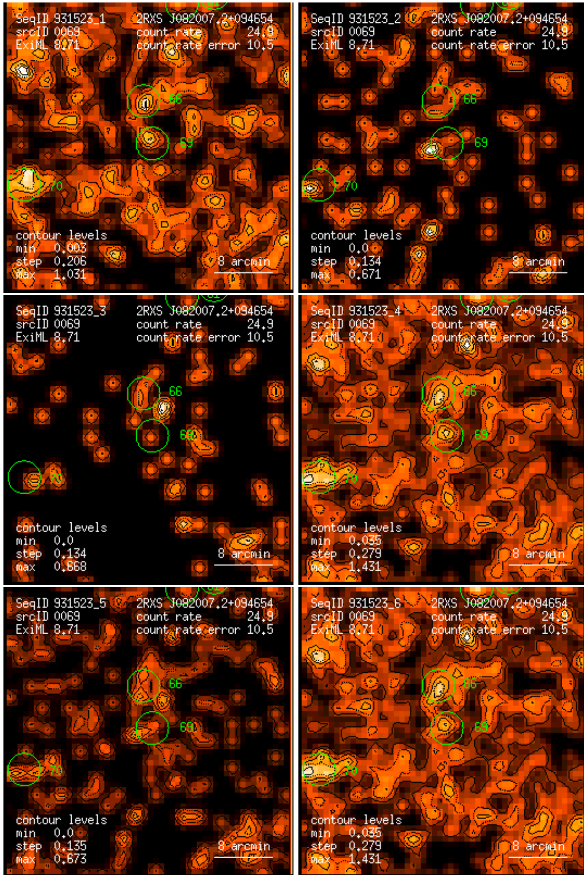
Figure 69: RASS 931523: detection 0069: band rate images, Gaussian filter: (1) PSPC channels 11 – 41, (2) 52 – 90, (3) 91 – 201, (4) 11 – 235, (5) 52 – 201, (6) 11 – 201. Broad band rates in counts/ks. Band rate contour levels in counts/ks/arcmin 2 .
