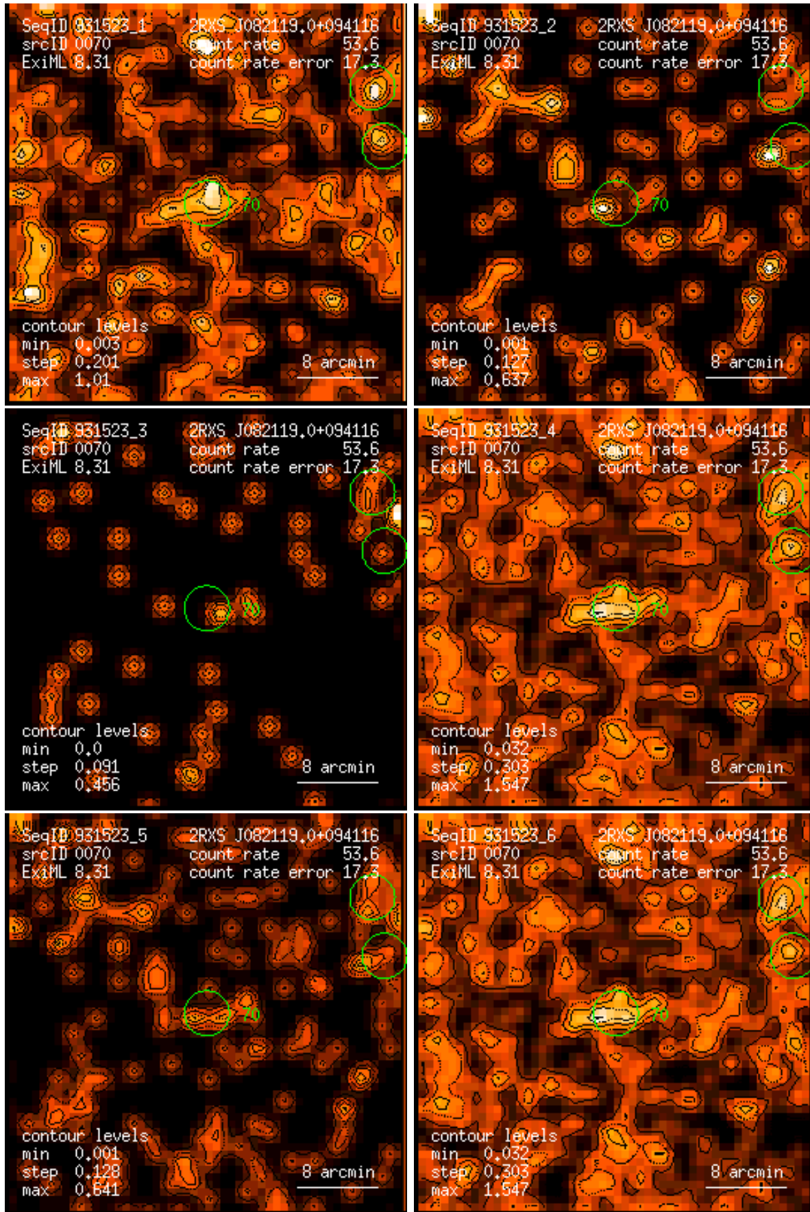
Figure 70: RASS 931523: detection 0070: band rate images, Gaussian filter: (1) PSPC channels 11 – 41, (2) 52 – 90, (3) 91 – 201, (4) 11 – 235, (5) 52 – 201, (6) 11 – 201. Broad band rates in counts/ks. Band rate contour levels in counts/ks/arcmin 2 .
