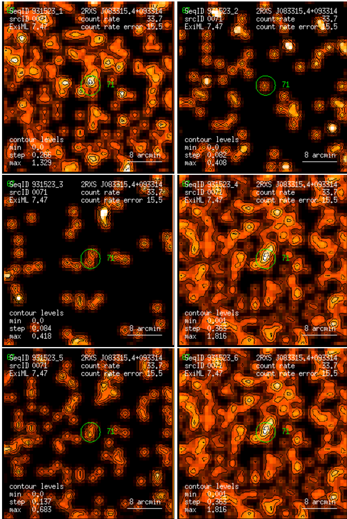
Figure 71: RASS 931523: detection 0071: band rate images, Gaussian filter: (1) PSPC channels 11 – 41, (2) 52 – 90, (3) 91 – 201, (4) 11 – 235, (5) 52 – 201, (6) 11 – 201. Broad band rates in counts/ks. Band rate contour levels in counts/ks/arcmin 2 .
