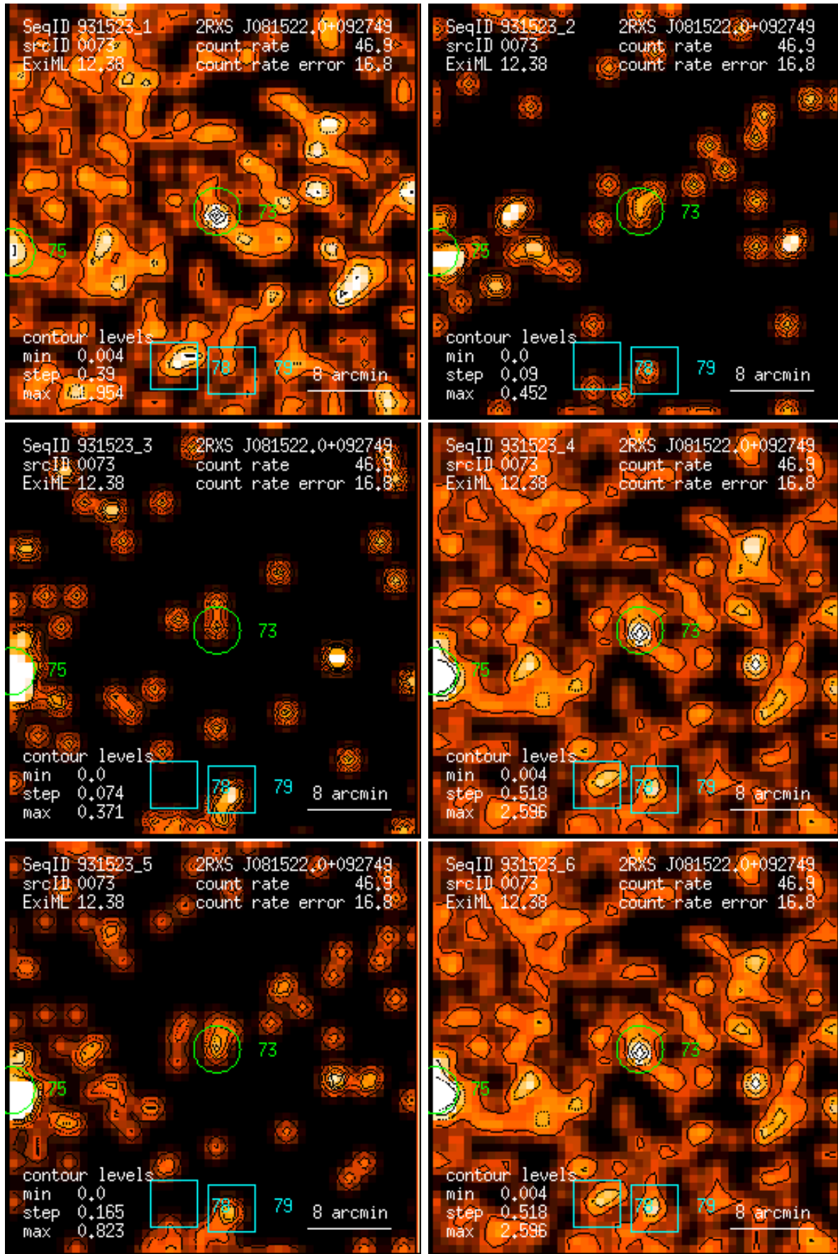
Figure 73: RASS 931523: detection 0073: band rate images, Gaussian filter: (1) PSPC channels 11 – 41, (2) 52 – 90, (3) 91 – 201, (4) 11 – 235, (5) 52 – 201, (6) 11 – 201. Broad band rates in counts/ks. Band rate contour levels in counts/ks/arcmin 2 .
