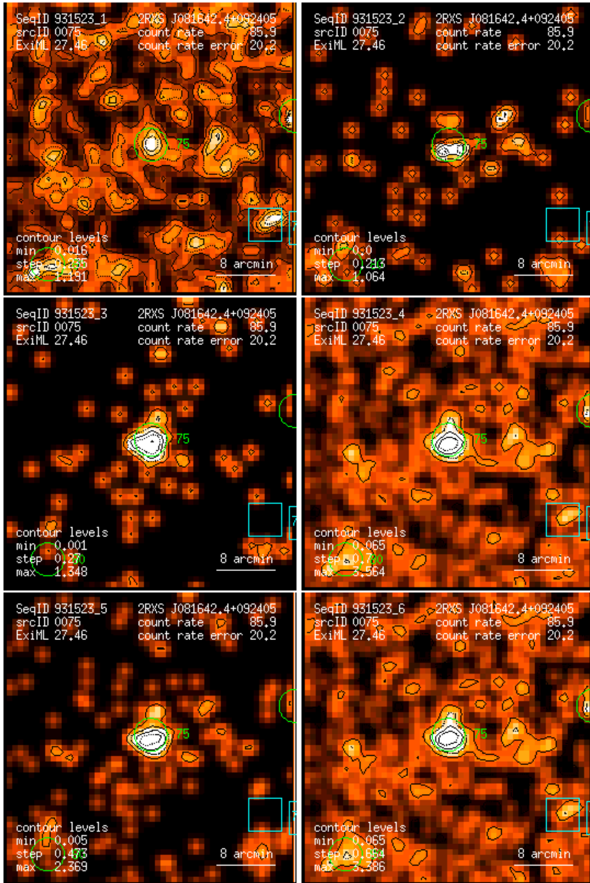
Figure 75: RASS 931523: detection 0075: band rate images, Gaussian filter: (1) PSPC channels 11 – 41, (2) 52 – 90, (3) 91 – 201, (4) 11 – 235, (5) 52 – 201, (6) 11 – 201. Broad band rates in counts/ks. Band rate contour levels in counts/ks/arcmin 2 .
