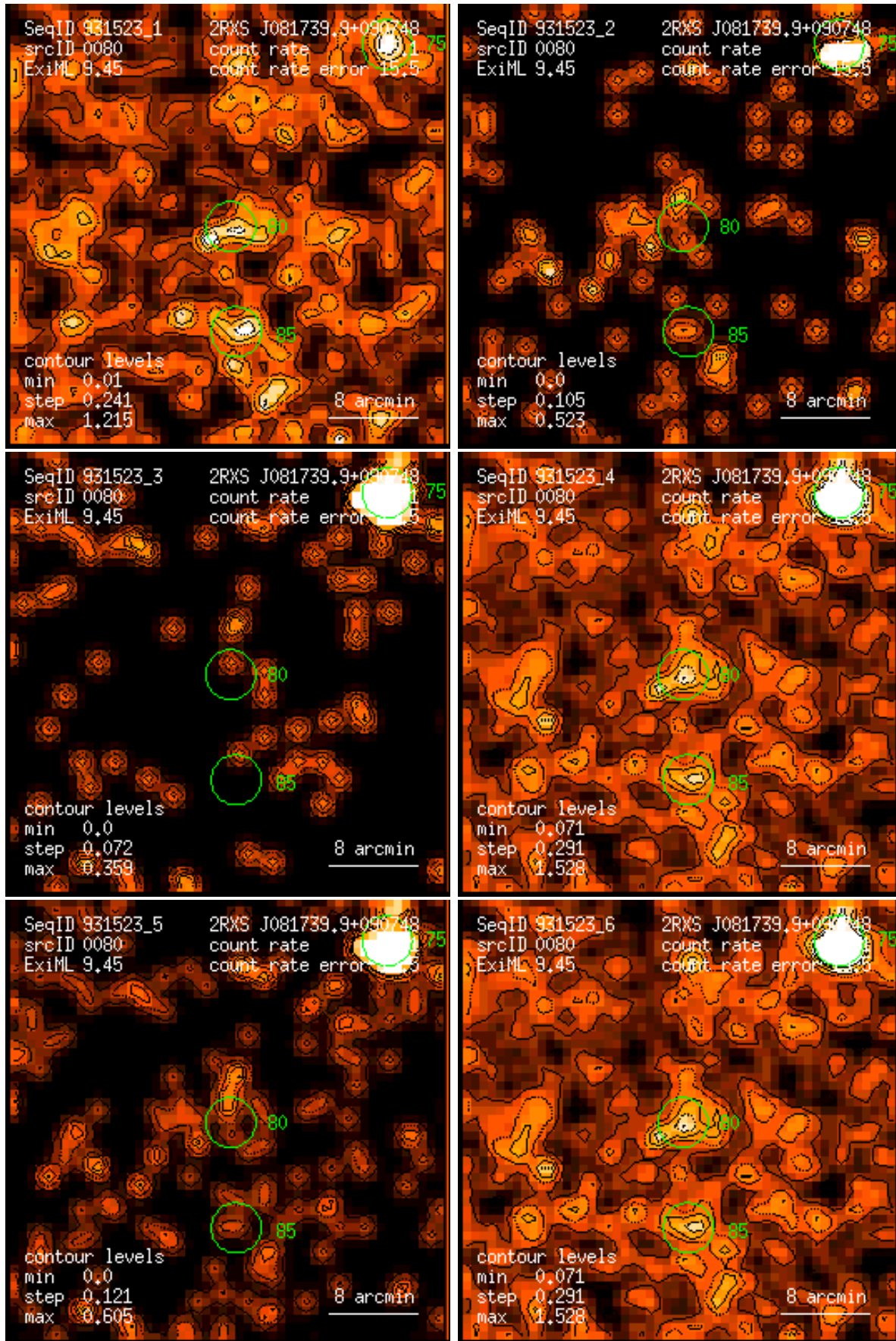
Figure 80: RASS 931523: detection 0080: band rate images, Gaussian filter: (1) PSPC channels 11 – 41, (2) 52 – 90, (3) 91 – 201, (4) 11 – 235, (5) 52 – 201, (6) 11 – 201. Broad band rates in counts/ks. Band rate contour levels in counts/ks/arcmin 2 .
