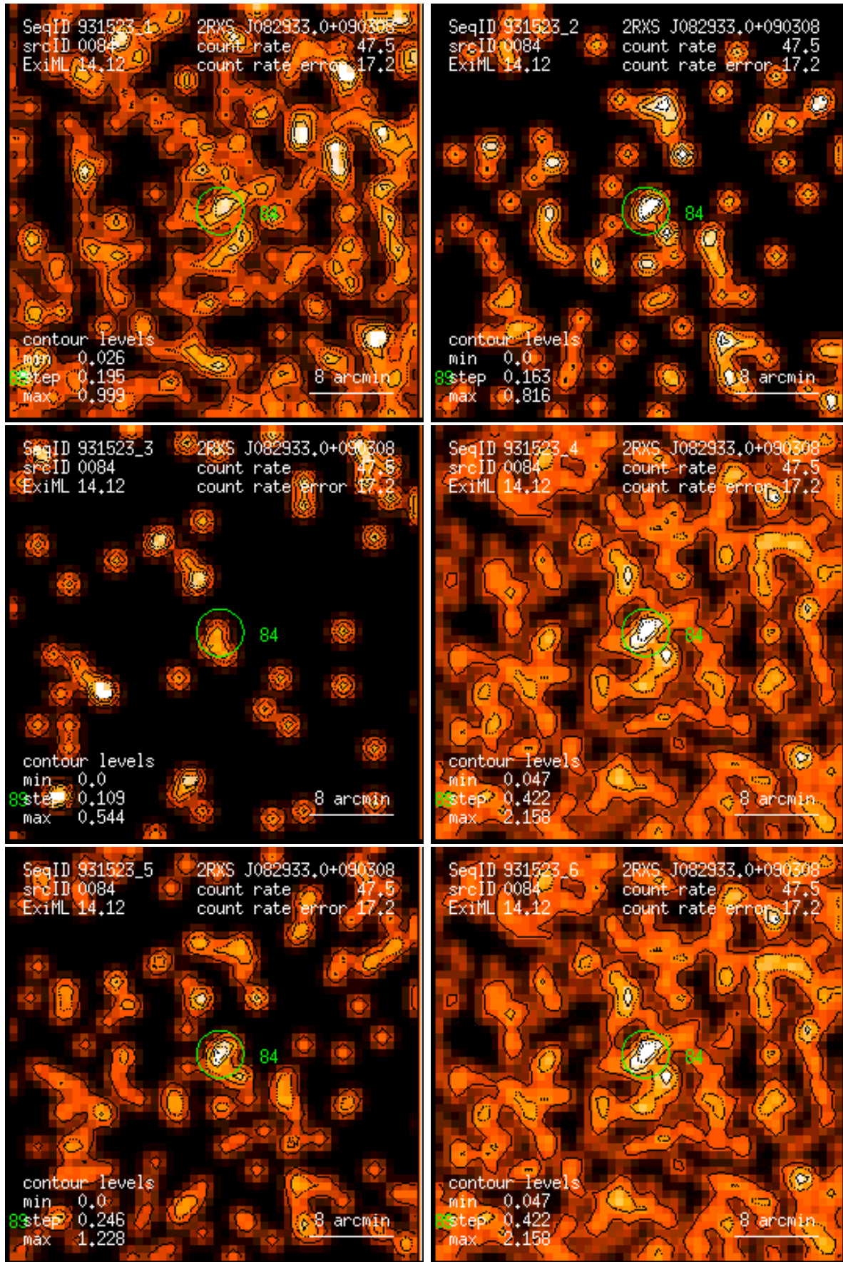
Figure 84: RASS 931523: detection 0084: band rate images, Gaussian filter: (1) PSPC channels 11 – 41, (2) 52 – 90, (3) 91 – 201, (4) 11 – 235, (5) 52 – 201, (6) 11 – 201. Broad band rates in counts/ks. Band rate contour levels in counts/ks/arcmin 2 .
