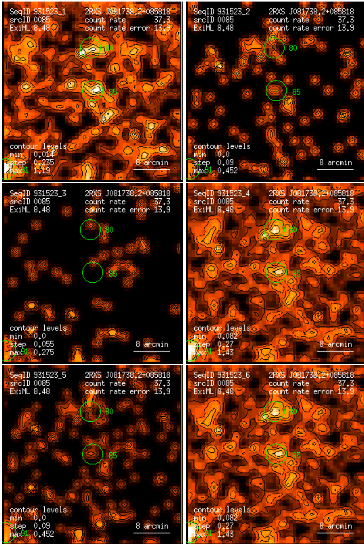
Figure 85: RASS 931523: detection 0085: band rate images, Gaussian filter: (1) PSPC channels 11 – 41, (2) 52 – 90, (3) 91 – 201, (4) 11 – 235, (5) 52 – 201, (6) 11 – 201. Broad band rates in counts/ks. Band rate contour levels in counts/ks/arcmin 2 .
