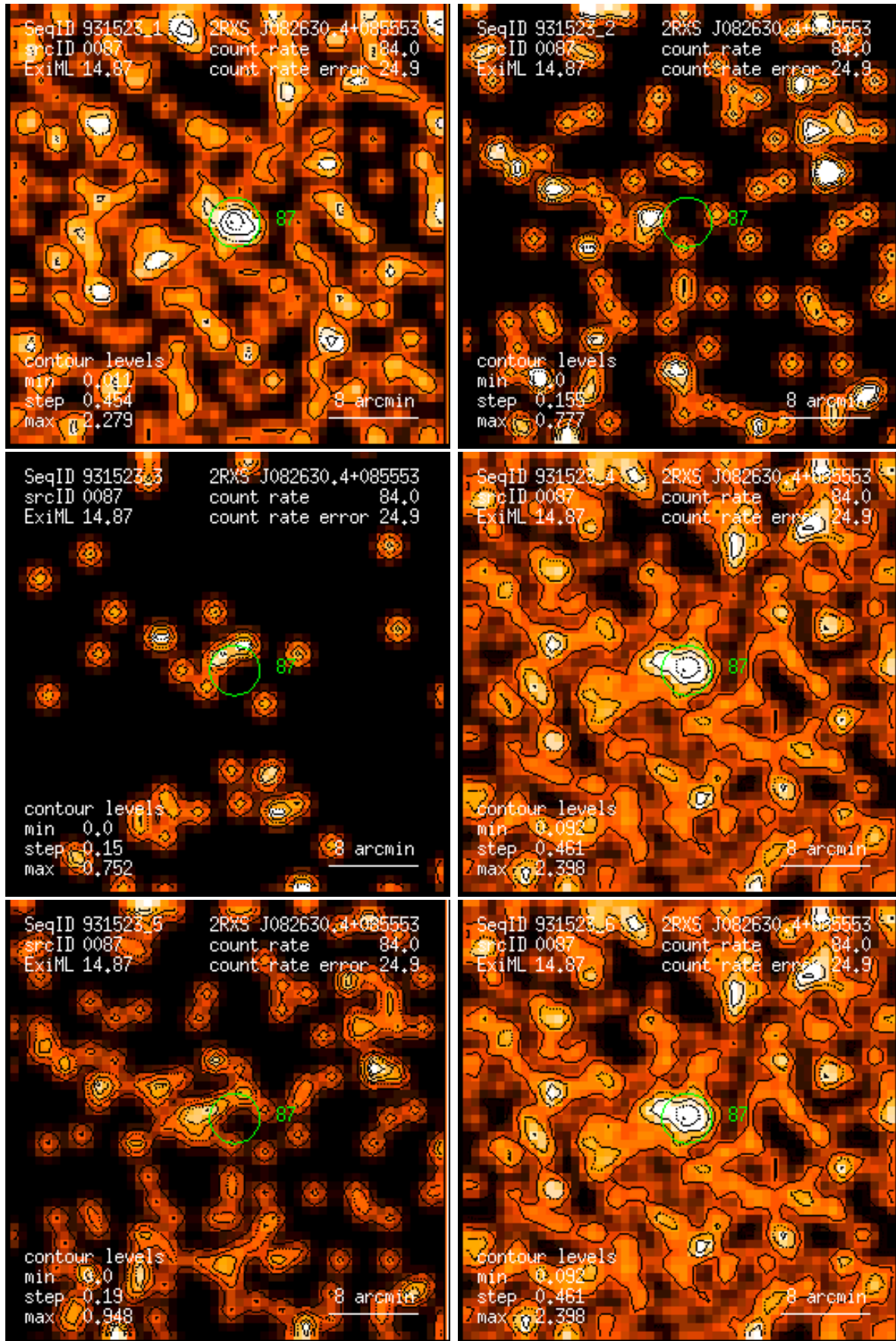
Figure 87: RASS 931523: detection 0087: band rate images, Gaussian filter: (1) PSPC channels 11 – 41, (2) 52 – 90, (3) 91 – 201, (4) 11 – 235, (5) 52 – 201, (6) 11 – 201. Broad band rates in counts/ks. Band rate contour levels in counts/ks/arcmin 2 .
