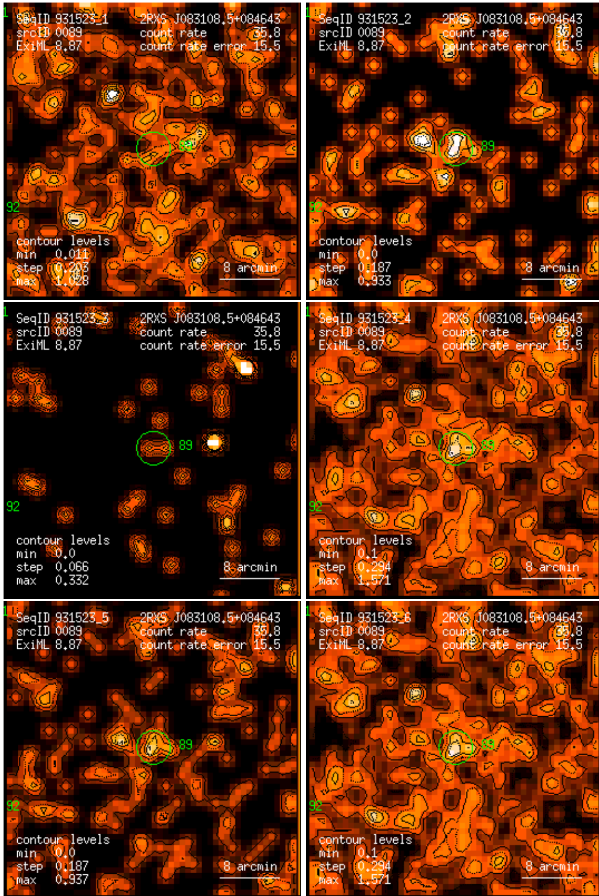
Figure 89: RASS 931523: detection 0089: band rate images, Gaussian filter: (1) PSPC channels 11 – 41, (2) 52 – 90, (3) 91 – 201, (4) 11 – 235, (5) 52 – 201, (6) 11 – 201. Broad band rates in counts/ks. Band rate contour levels in counts/ks/arcmin 2 .
