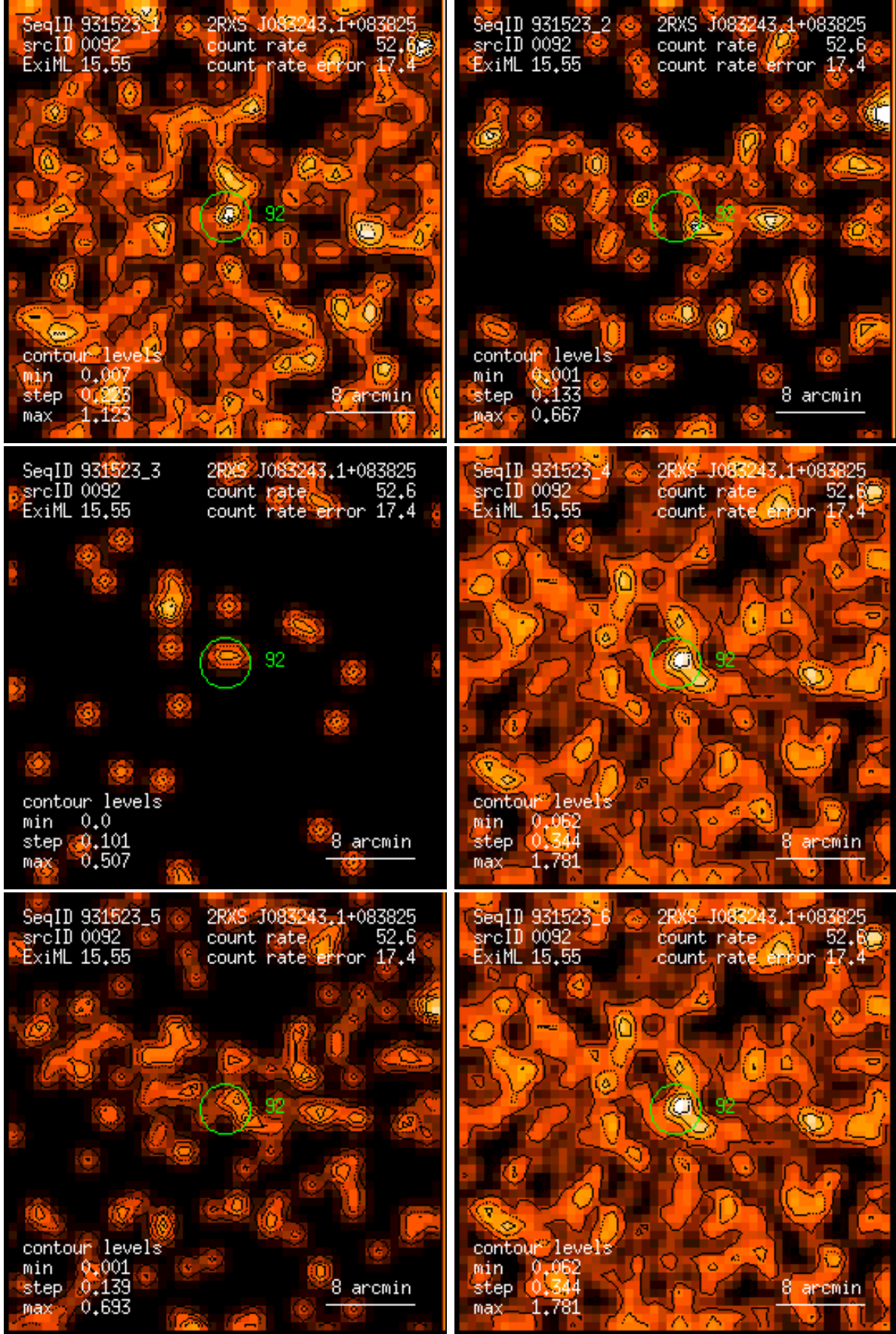
Figure 92: RASS 931523: detection 0092: band rate images, Gaussian filter: (1) PSPC channels 11 – 41, (2) 52 – 90, (3) 91 – 201, (4) 11 – 235, (5) 52 – 201, (6) 11 – 201. Broad band rates in counts/ks. Band rate contour levels in counts/ks/arcmin 2 .
