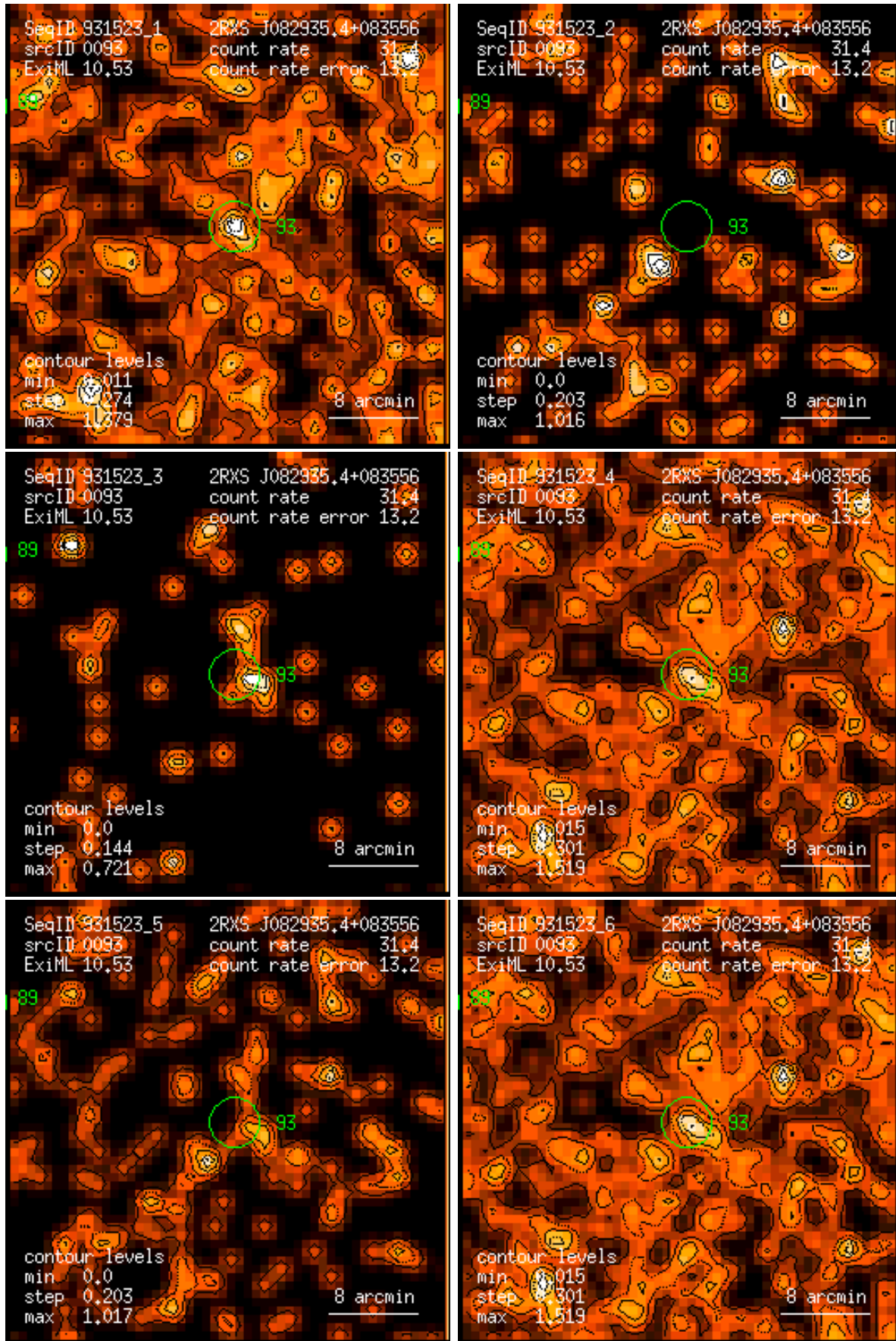
Figure 93: RASS 931523: detection 0093: band rate images, Gaussian filter: (1) PSPC channels 11 – 41, (2) 52 – 90, (3) 91 – 201, (4) 11 – 235, (5) 52 – 201, (6) 11 – 201. Broad band rates in counts/ks. Band rate contour levels in counts/ks/arcmin 2 .
