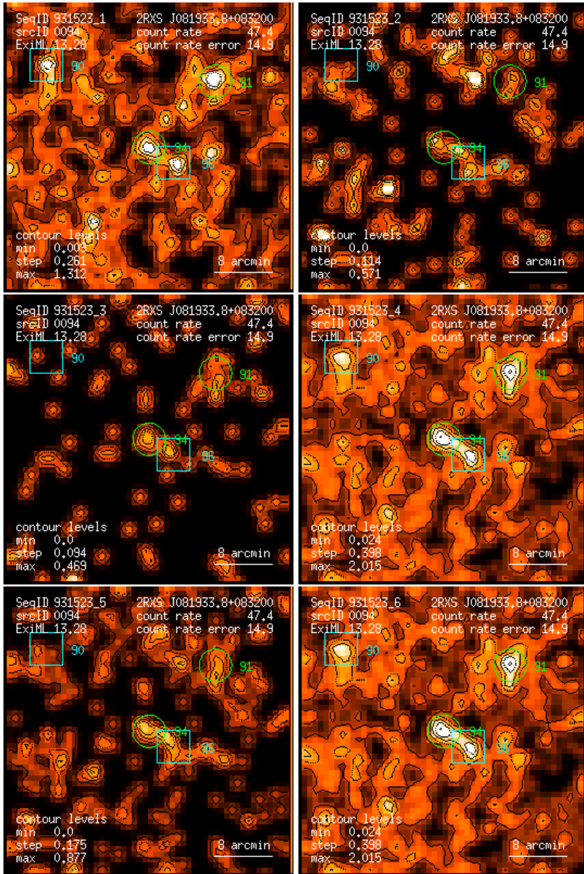
Figure 94: RASS 931523: detection 0094: band rate images, Gaussian filter: (1) PSPC channels 11 – 41, (2) 52 – 90, (3) 91 – 201, (4) 11 – 235, (5) 52 – 201, (6) 11 – 201. Broad band rates in counts/ks. Band rate contour levels in counts/ks/arcmin 2 .
