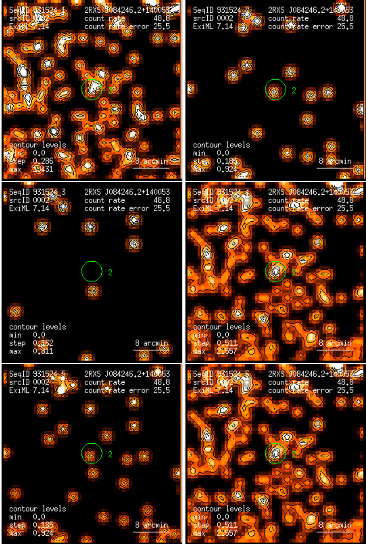
Figure 2: RASS 931524: detection 0002: band rate images, Gaussian filter: (1) PSPC channels 11 – 41, (2) 52 – 90, (3) 91 – 201, (4) 11 – 235, (5) 52 – 201, (6) 11 – 201. Broad band rates in counts/ks. Band rate contour levels in counts/ks/arcmin 2 .
