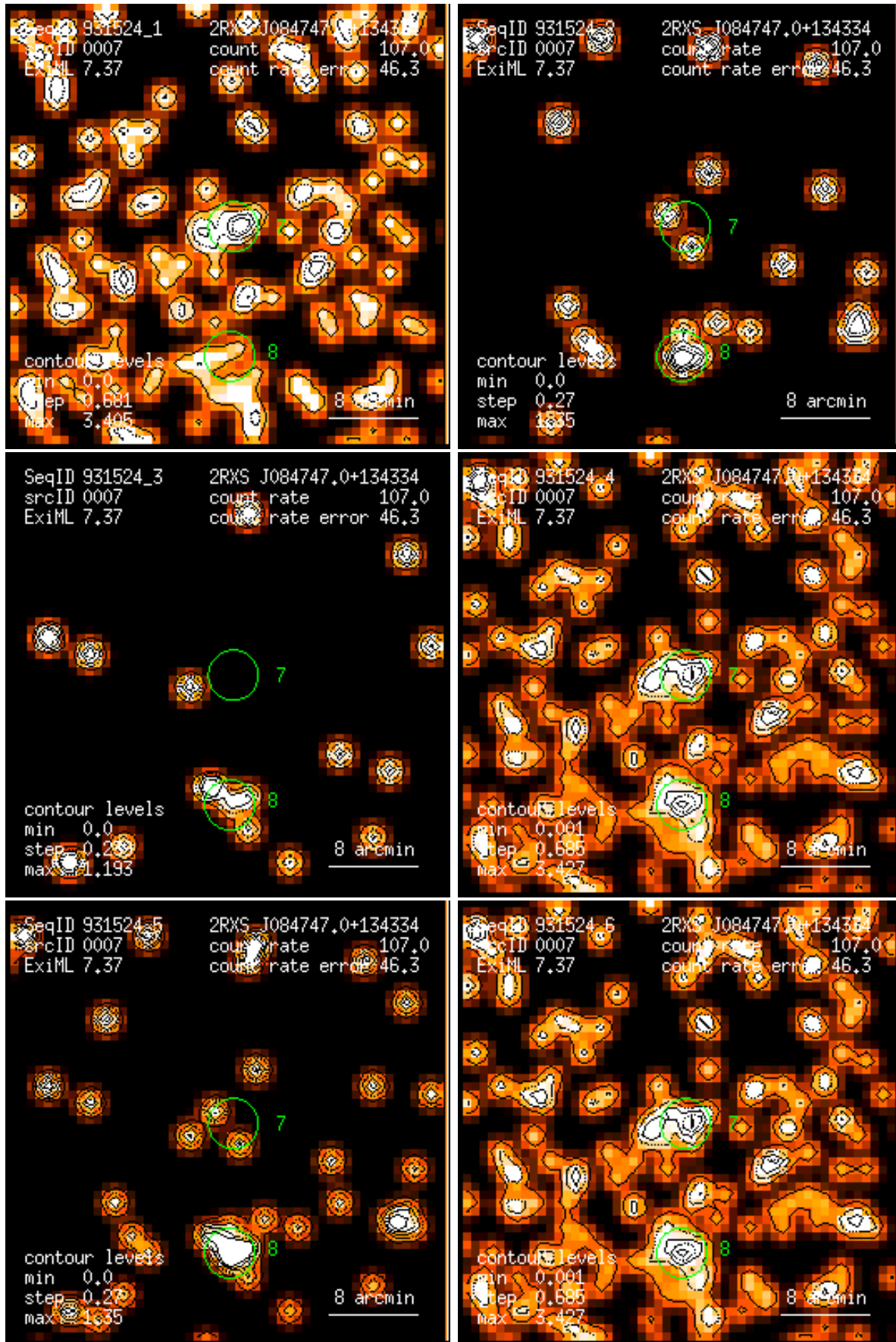
Figure 7: RASS 931524: detection 0007: band rate images, Gaussian filter: (1) PSPC channels 11 – 41, (2) 52 – 90, (3) 91 – 201, (4) 11 – 235, (5) 52 – 201, (6) 11 – 201. Broad band rates in counts/ks. Band rate contour levels in counts/ks/arcmin 2 .
