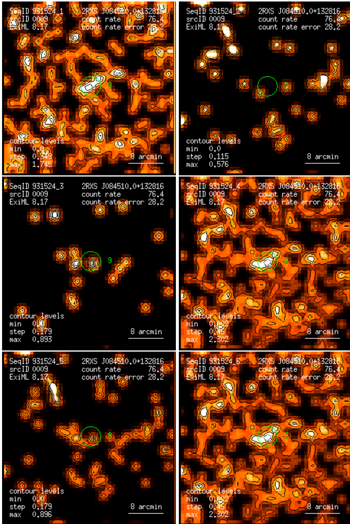
Figure 9: RASS 931524: detection 0009: band rate images, Gaussian filter: (1) PSPC channels 11 – 41, (2) 52 – 90, (3) 91 – 201, (4) 11 – 235, (5) 52 – 201, (6) 11 – 201. Broad band rates in counts/ks. Band rate contour levels in counts/ks/arcmin 2 .
