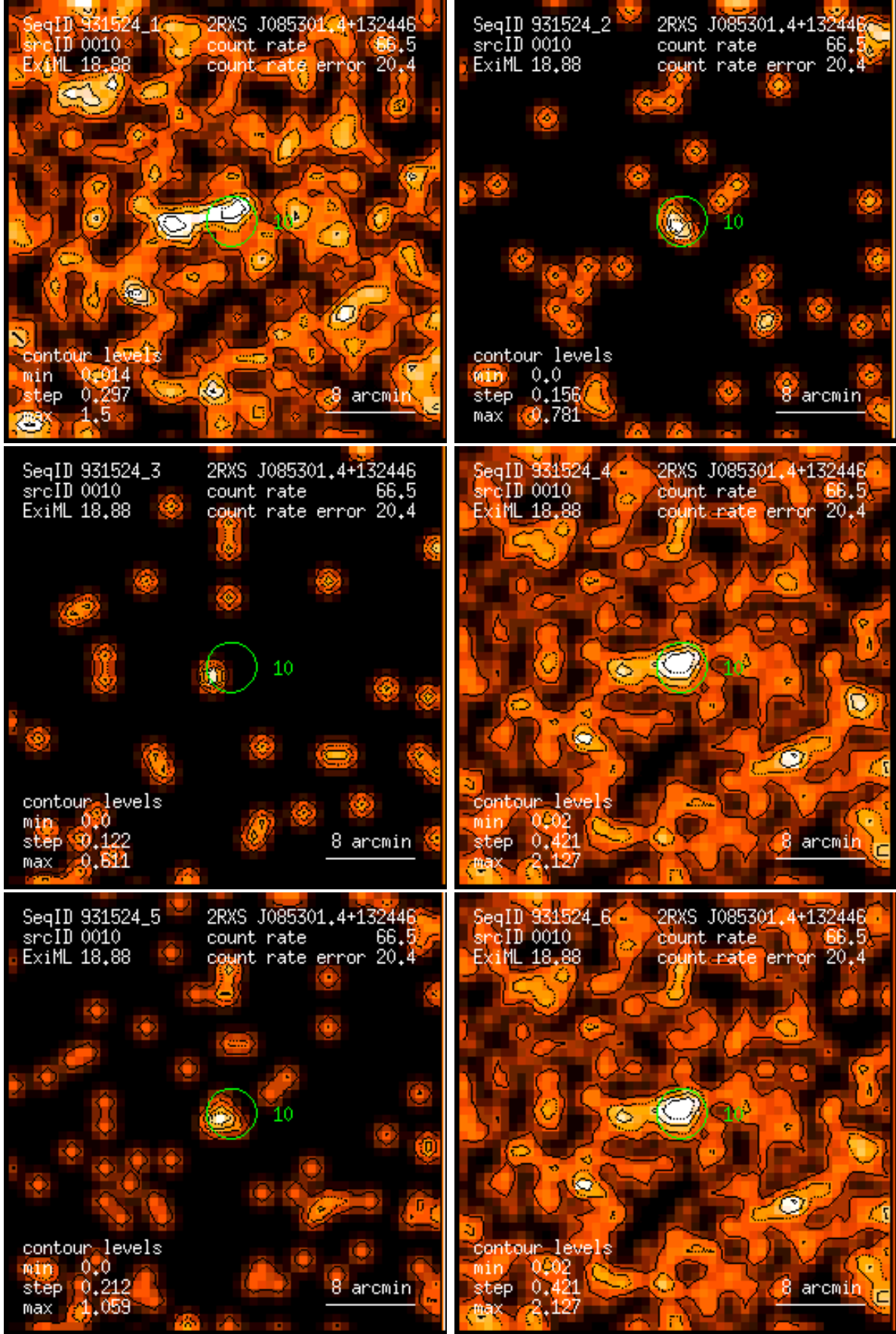
Figure 10: RASS 931524: detection 0010: band rate images, Gaussian filter: (1) PSPC channels 11 – 41, (2) 52 – 90, (3) 91 – 201, (4) 11 – 235, (5) 52 – 201, (6) 11 – 201. Broad band rates in counts/ks. Band rate contour levels in counts/ks/arcmin 2 .
