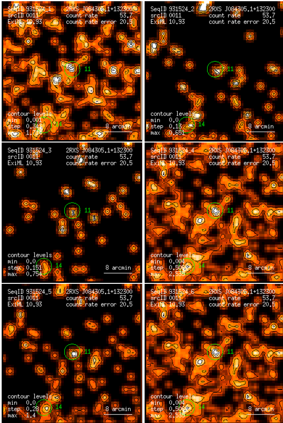
Figure 11: RASS 931524: detection 0011: band rate images, Gaussian filter: (1) PSPC channels 11 – 41, (2) 52 – 90, (3) 91 – 201, (4) 11 – 235, (5) 52 – 201, (6) 11 – 201. Broad band rates in counts/ks. Band rate contour levels in counts/ks/arcmin 2 .
