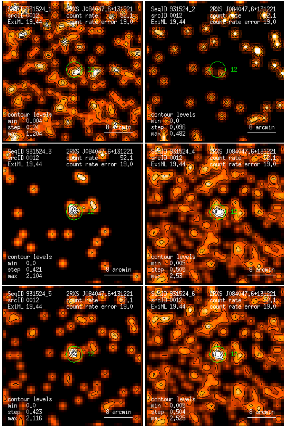
Figure 12: RASS 931524: detection 0012: band rate images, Gaussian filter: (1) PSPC channels 11 – 41, (2) 52 – 90, (3) 91 – 201, (4) 11 – 235, (5) 52 – 201, (6) 11 – 201. Broad band rates in counts/ks. Band rate contour levels in counts/ks/arcmin 2 .
