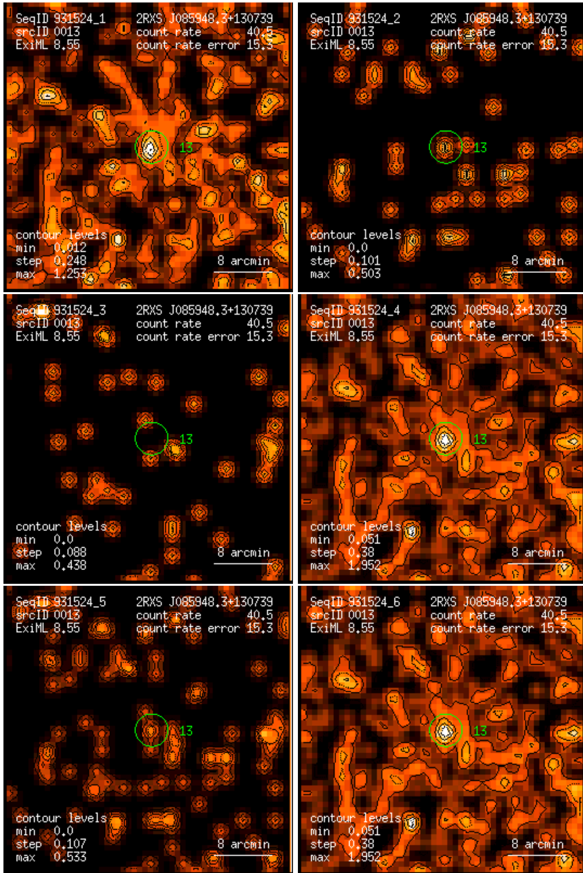
Figure 13: RASS 931524: detection 0013: band rate images, Gaussian filter: (1) PSPC channels 11 – 41, (2) 52 – 90, (3) 91 – 201, (4) 11 – 235, (5) 52 – 201, (6) 11 – 201. Broad band rates in counts/ks. Band rate contour levels in counts/ks/arcmin 2 .
