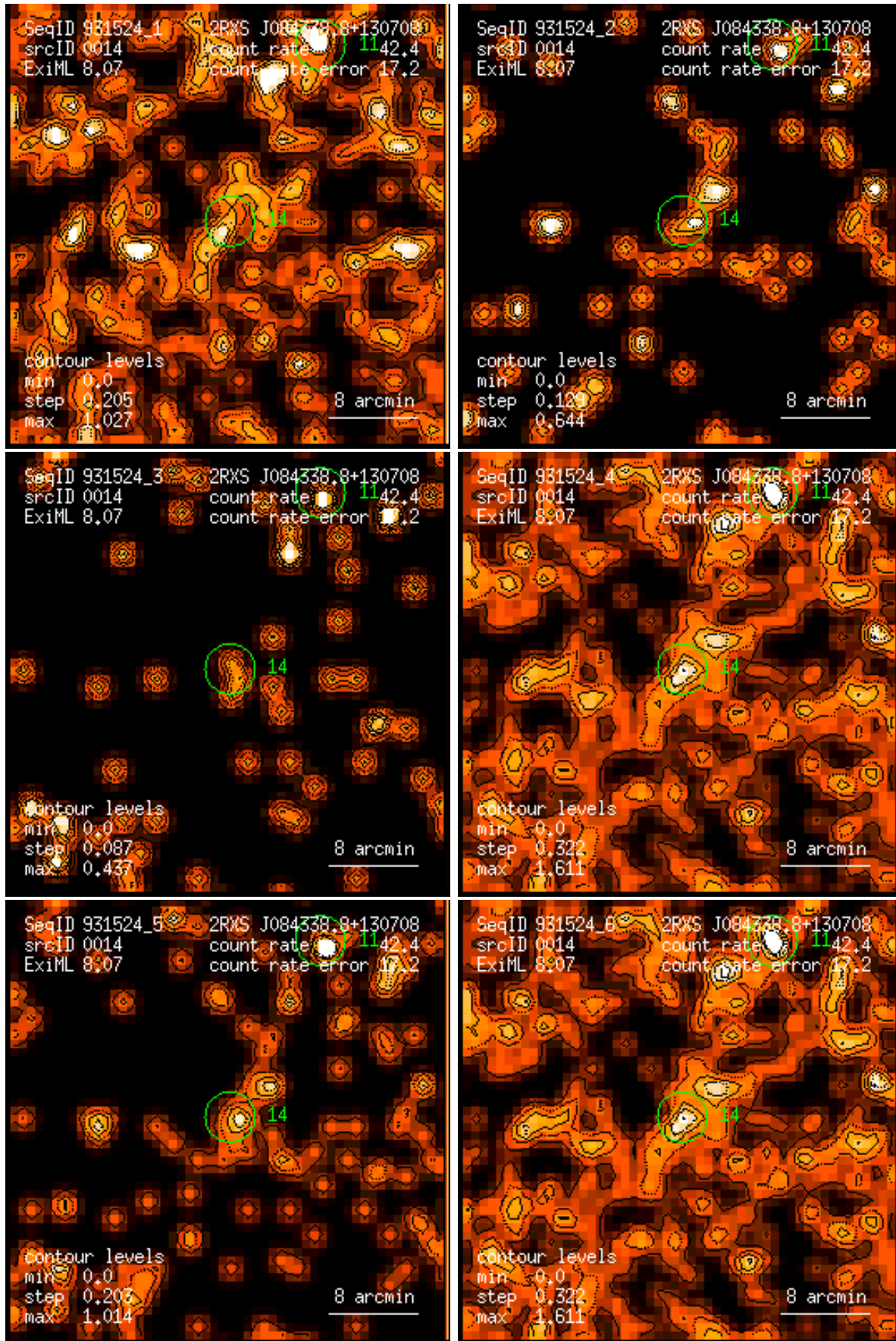
Figure 14: RASS 931524: detection 0014: band rate images, Gaussian filter: (1) PSPC channels 11 – 41, (2) 52 – 90, (3) 91 – 201, (4) 11 – 235, (5) 52 – 201, (6) 11 – 201. Broad band rates in counts/ks. Band rate contour levels in counts/ks/arcmin 2 .
