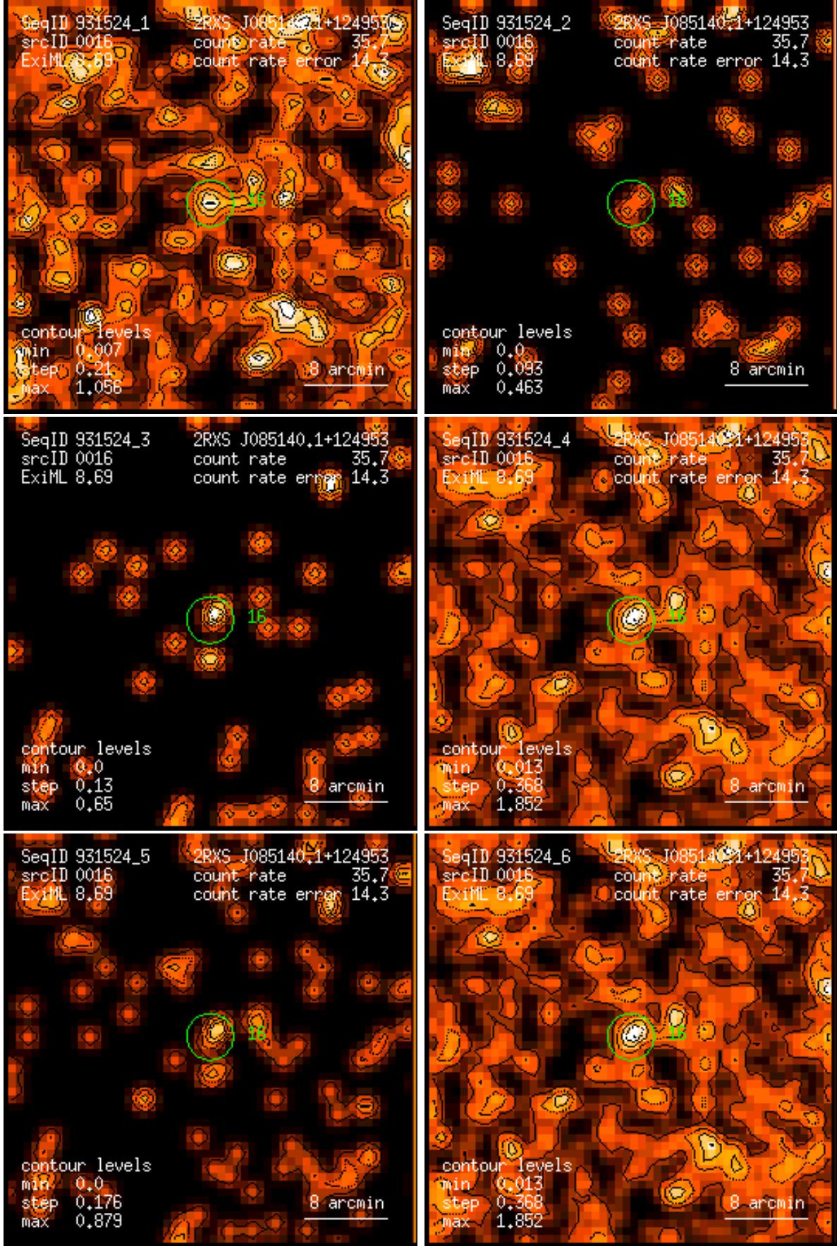
Figure 16: RASS 931524: detection 0016: band rate images, Gaussian filter: (1) PSPC channels 11 – 41, (2) 52 – 90, (3) 91 – 201, (4) 11 – 235, (5) 52 – 201, (6) 11 – 201. Broad band rates in counts/ks. Band rate contour levels in counts/ks/arcmin 2 .
