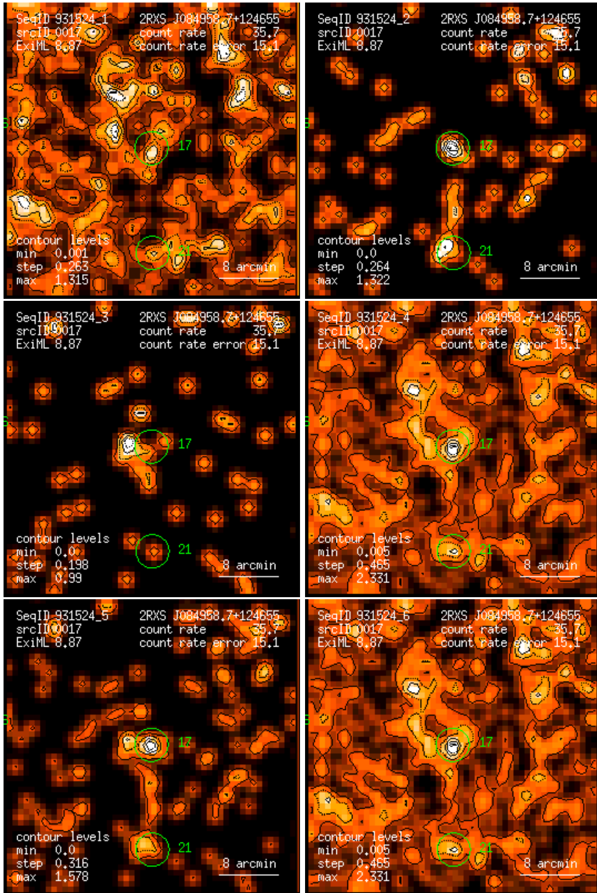
Figure 17: RASS 931524: detection 0017: band rate images, Gaussian filter: (1) PSPC channels 11 – 41, (2) 52 – 90, (3) 91 – 201, (4) 11 – 235, (5) 52 – 201, (6) 11 – 201. Broad band rates in counts/ks. Band rate contour levels in counts/ks/arcmin 2 .
