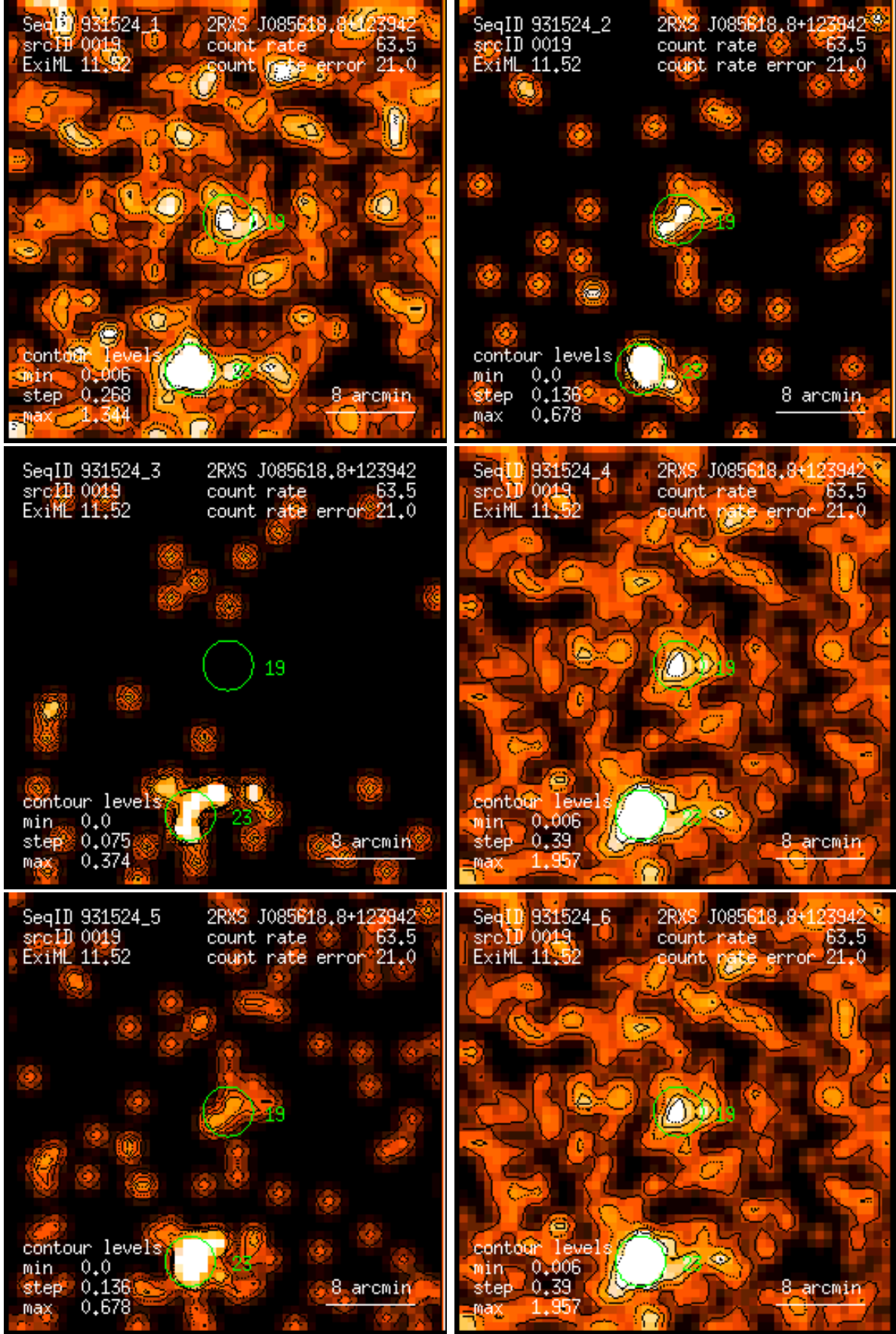
Figure 19: RASS 931524: detection 0019: band rate images, Gaussian filter: (1) PSPC channels 11 – 41, (2) 52 – 90, (3) 91 – 201, (4) 11 – 235, (5) 52 – 201, (6) 11 – 201. Broad band rates in counts/ks. Band rate contour levels in counts/ks/arcmin 2 .
