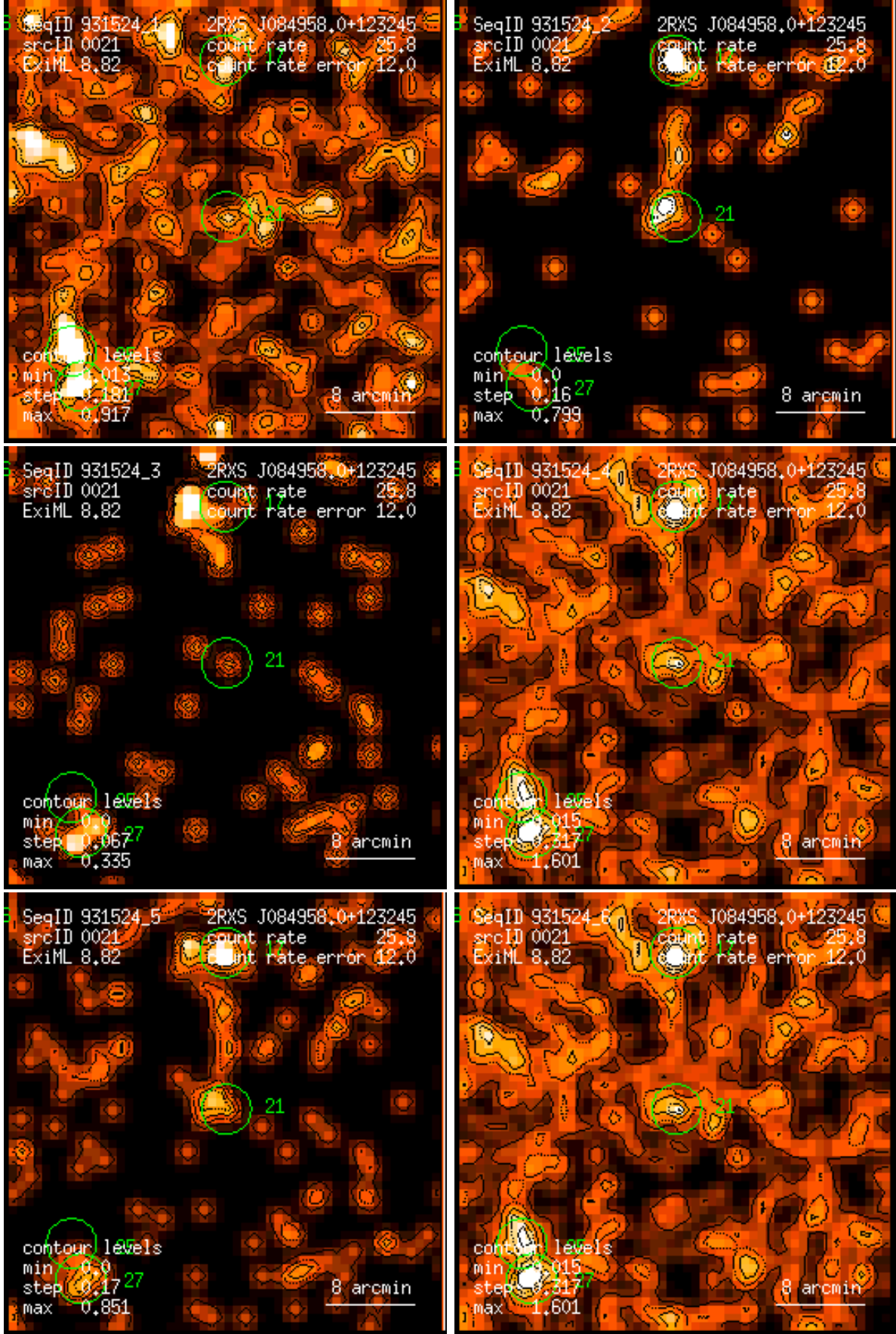
Figure 21: RASS 931524: detection 0021: band rate images, Gaussian filter: (1) PSPC channels 11 – 41, (2) 52 – 90, (3) 91 – 201, (4) 11 – 235, (5) 52 – 201, (6) 11 – 201. Broad band rates in counts/ks. Band rate contour levels in counts/ks/arcmin 2 .
