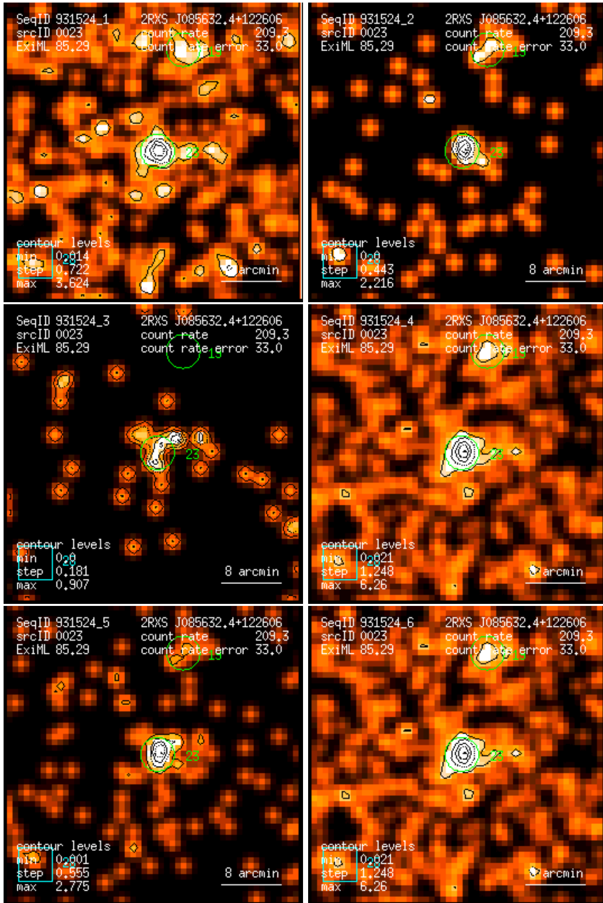
Figure 23: RASS 931524: detection 0023: band rate images, Gaussian filter: (1) PSPC channels 11 – 41, (2) 52 – 90, (3) 91 – 201, (4) 11 – 235, (5) 52 – 201, (6) 11 – 201. Broad band rates in counts/ks. Band rate contour levels in counts/ks/arcmin 2 .
