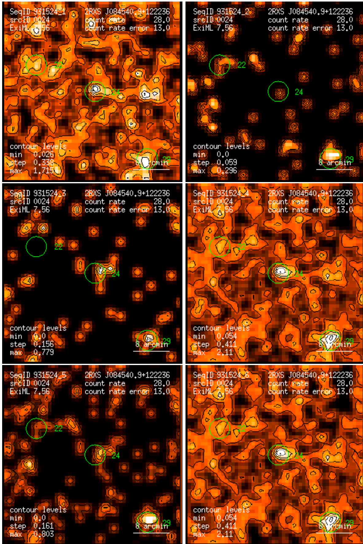
Figure 24: RASS 931524: detection 0024: band rate images, Gaussian filter: (1) PSPC channels 11 – 41, (2) 52 – 90, (3) 91 – 201, (4) 11 – 235, (5) 52 – 201, (6) 11 – 201. Broad band rates in counts/ks. Band rate contour levels in counts/ks/arcmin 2 .
