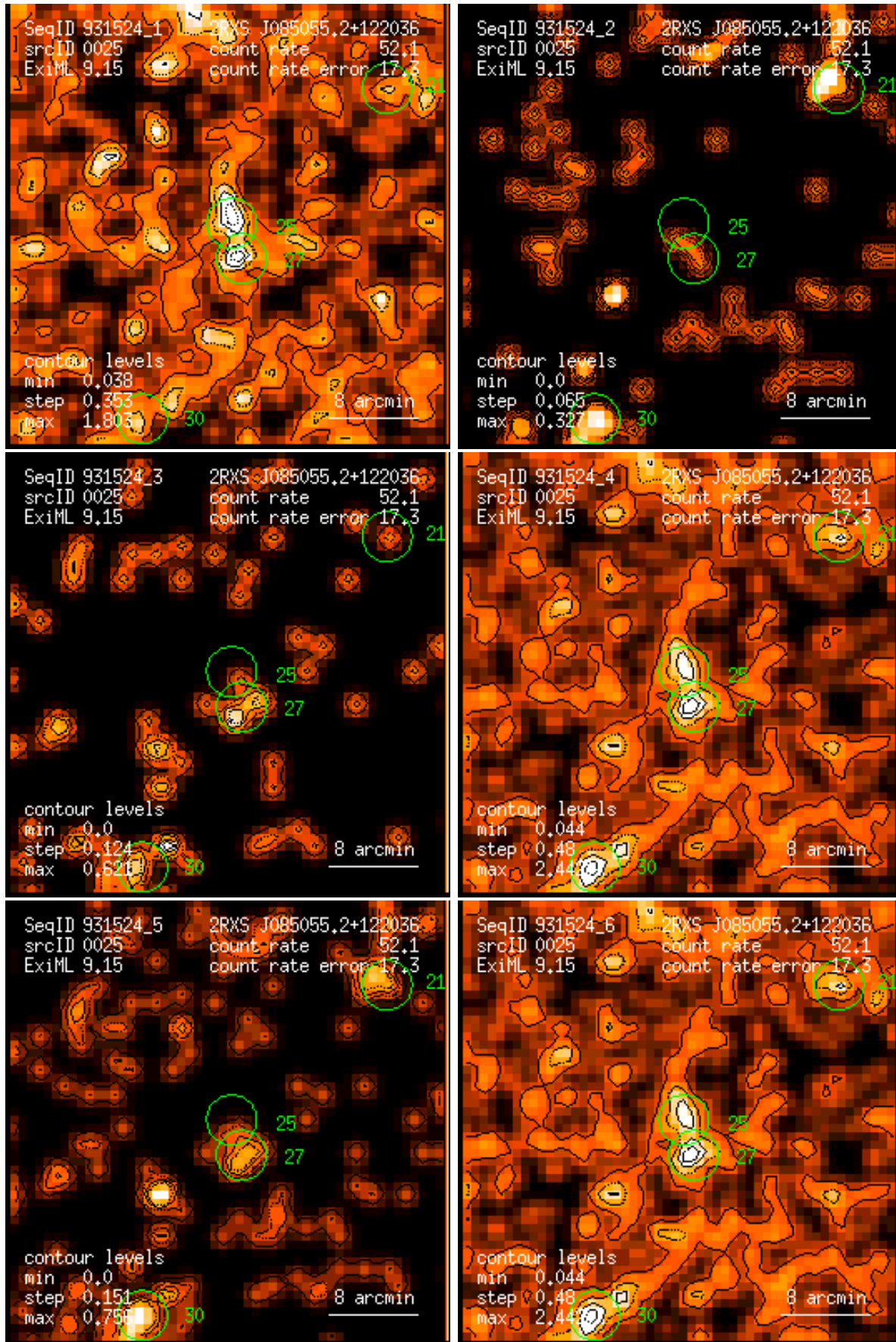
Figure 25: RASS 931524: detection 0025: band rate images, Gaussian filter: (1) PSPC channels 11 – 41, (2) 52 – 90, (3) 91 – 201, (4) 11 – 235, (5) 52 – 201, (6) 11 – 201. Broad band rates in counts/ks. Band rate contour levels in counts/ks/arcmin 2 .
