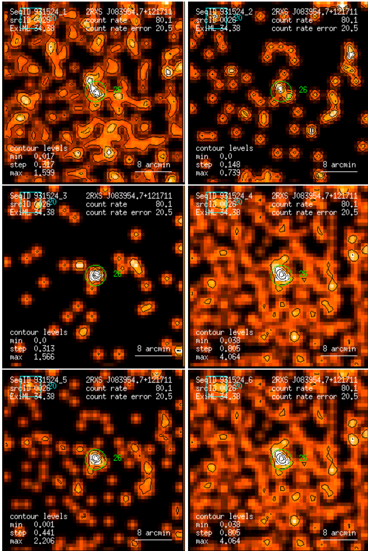
Figure 26: RASS 931524: detection 0026: band rate images, Gaussian filter: (1) PSPC channels 11 – 41, (2) 52 – 90, (3) 91 – 201, (4) 11 – 235, (5) 52 – 201, (6) 11 – 201. Broad band rates in counts/ks. Band rate contour levels in counts/ks/arcmin 2 .
