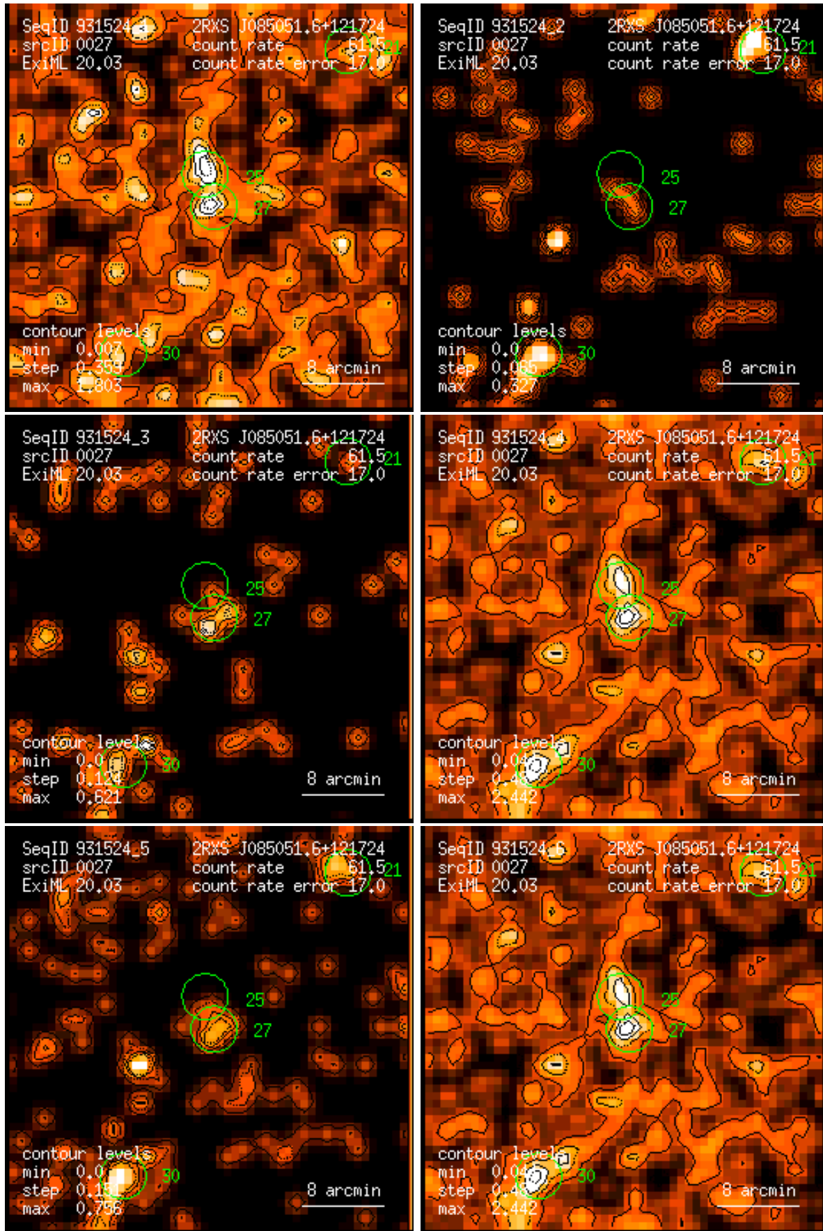
Figure 27: RASS 931524: detection 0027: band rate images, Gaussian filter: (1) PSPC channels 11 – 41, (2) 52 – 90, (3) 91 – 201, (4) 11 – 235, (5) 52 – 201, (6) 11 – 201. Broad band rates in counts/ks. Band rate contour levels in counts/ks/arcmin 2 .
