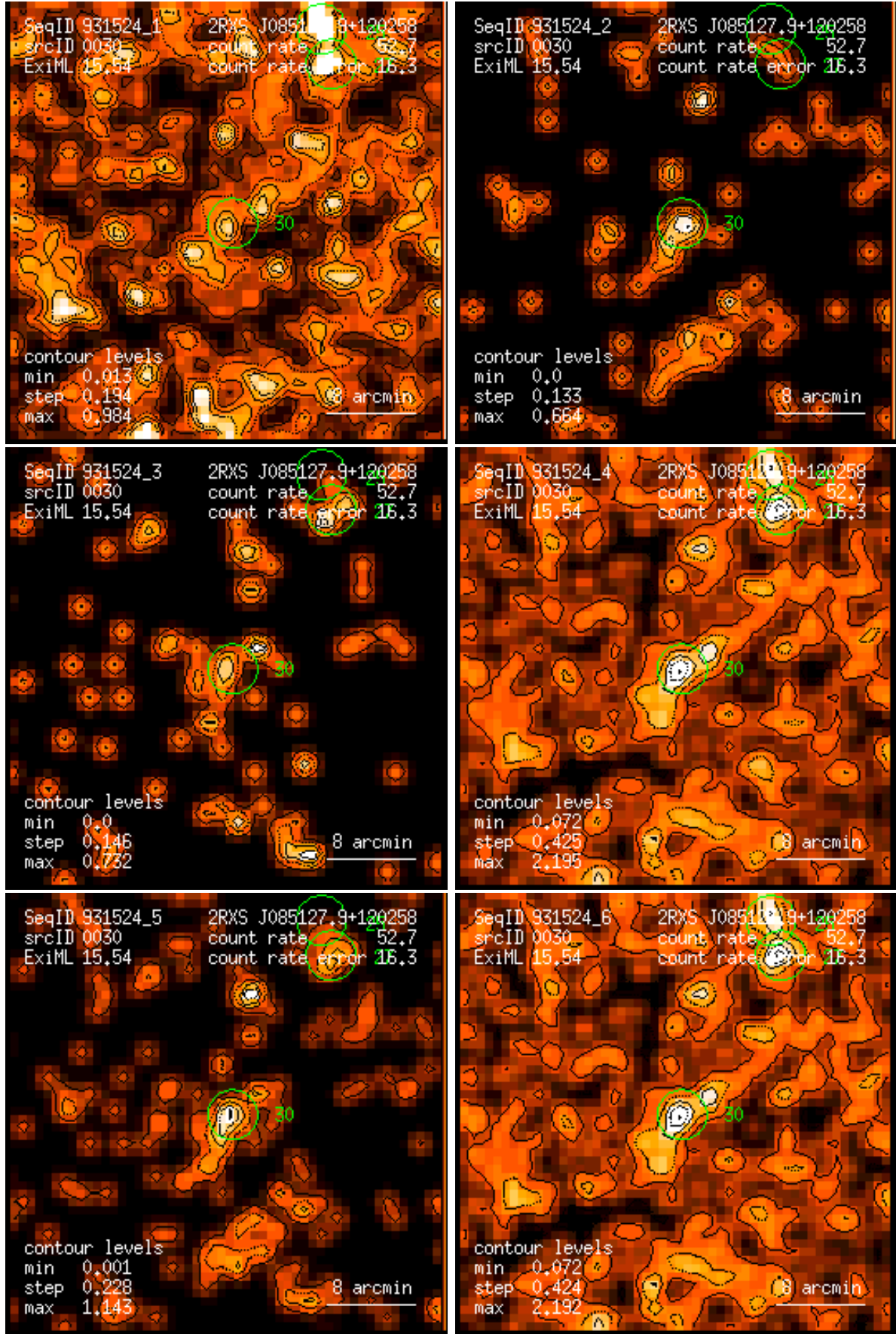
Figure 30: RASS 931524: detection 0030: band rate images, Gaussian filter: (1) PSPC channels 11 – 41, (2) 52 – 90, (3) 91 – 201, (4) 11 – 235, (5) 52 – 201, (6) 11 – 201. Broad band rates in counts/ks. Band rate contour levels in counts/ks/arcmin 2 .
