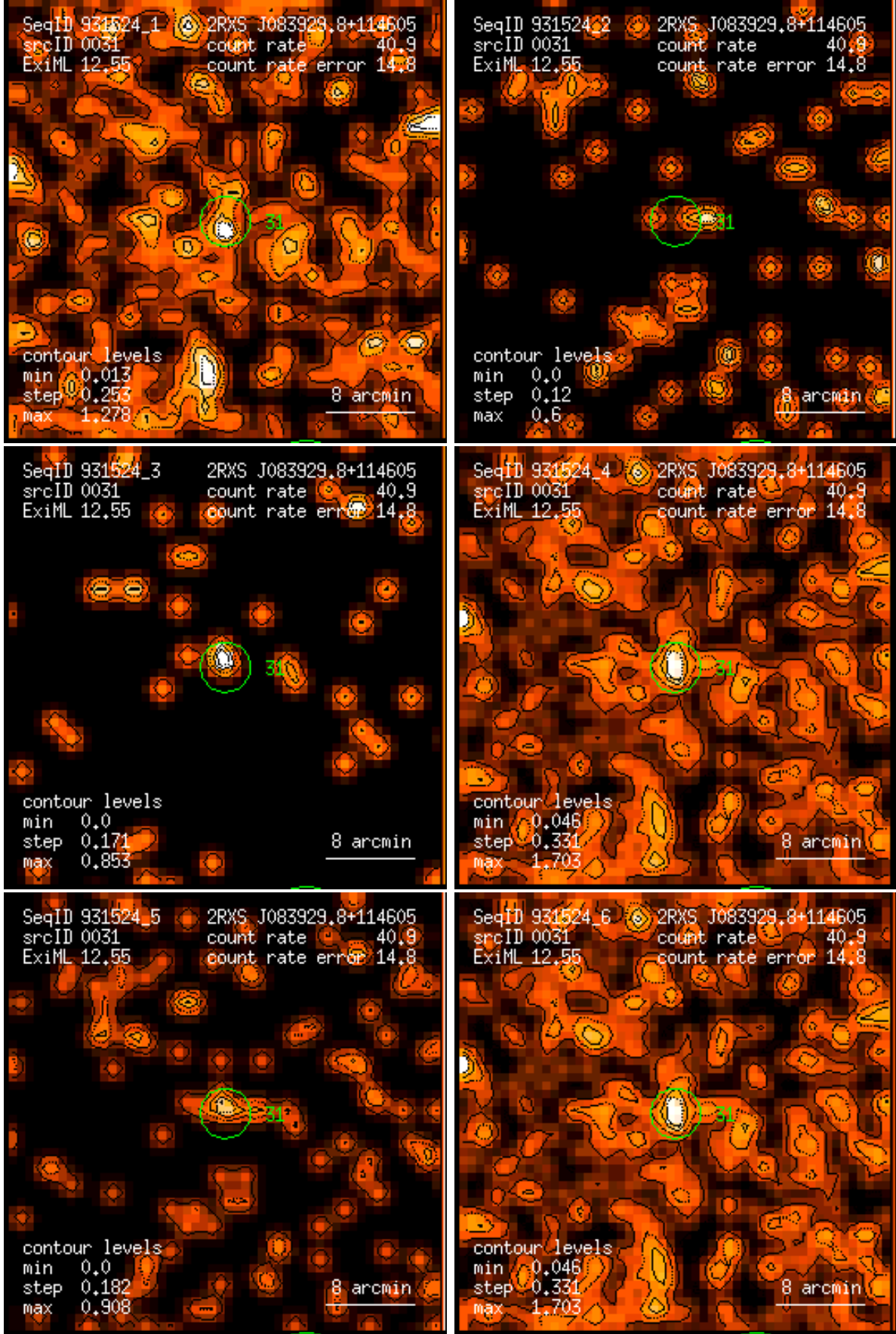
Figure 31: RASS 931524: detection 0031: band rate images, Gaussian filter: (1) PSPC channels 11 – 41, (2) 52 – 90, (3) 91 – 201, (4) 11 – 235, (5) 52 – 201, (6) 11 – 201. Broad band rates in counts/ks. Band rate contour levels in counts/ks/arcmin 2 .
