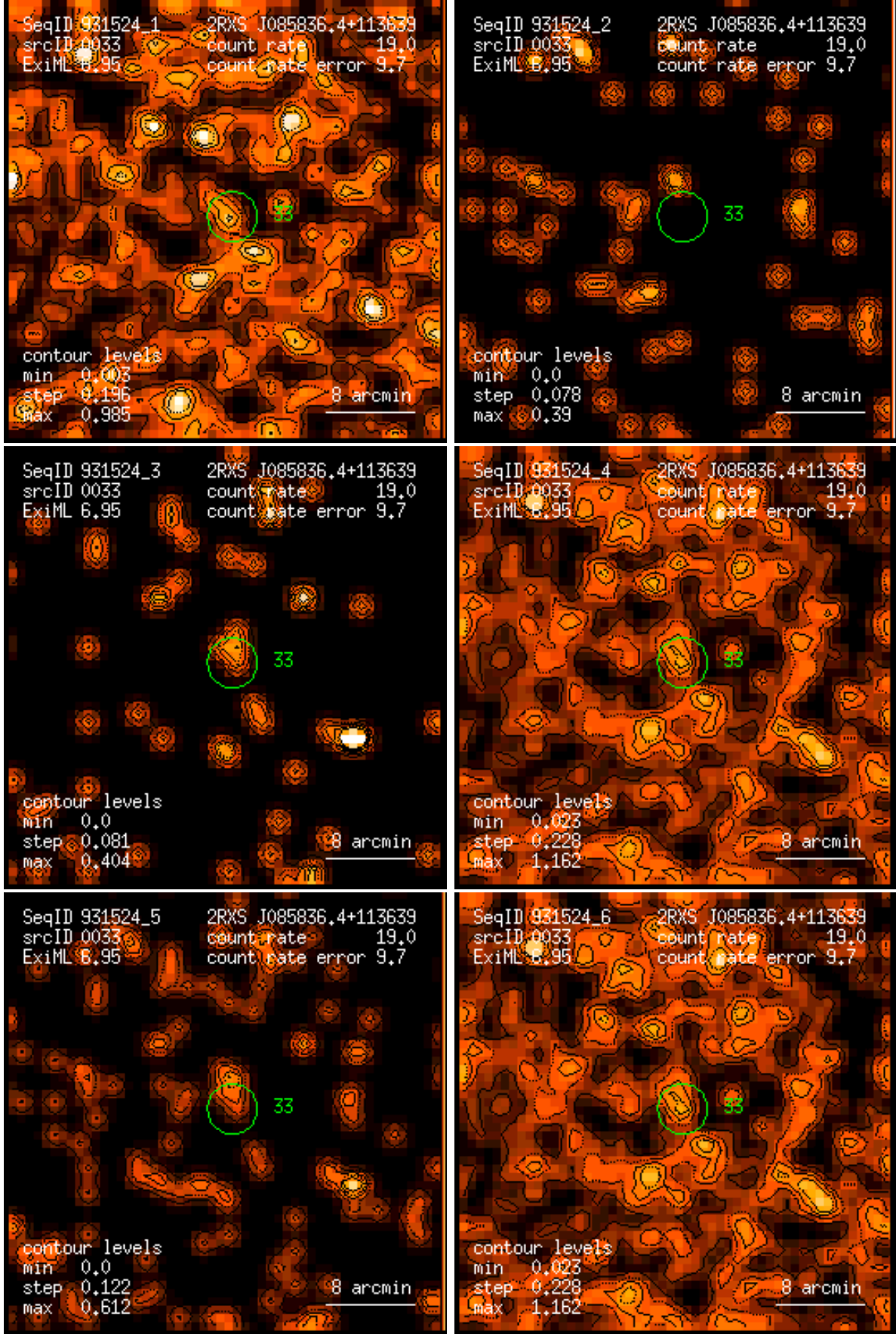
Figure 33: RASS 931524: detection 0033: band rate images, Gaussian filter: (1) PSPC channels 11 – 41, (2) 52 – 90, (3) 91 – 201, (4) 11 – 235, (5) 52 – 201, (6) 11 – 201. Broad band rates in counts/ks. Band rate contour levels in counts/ks/arcmin 2 .
