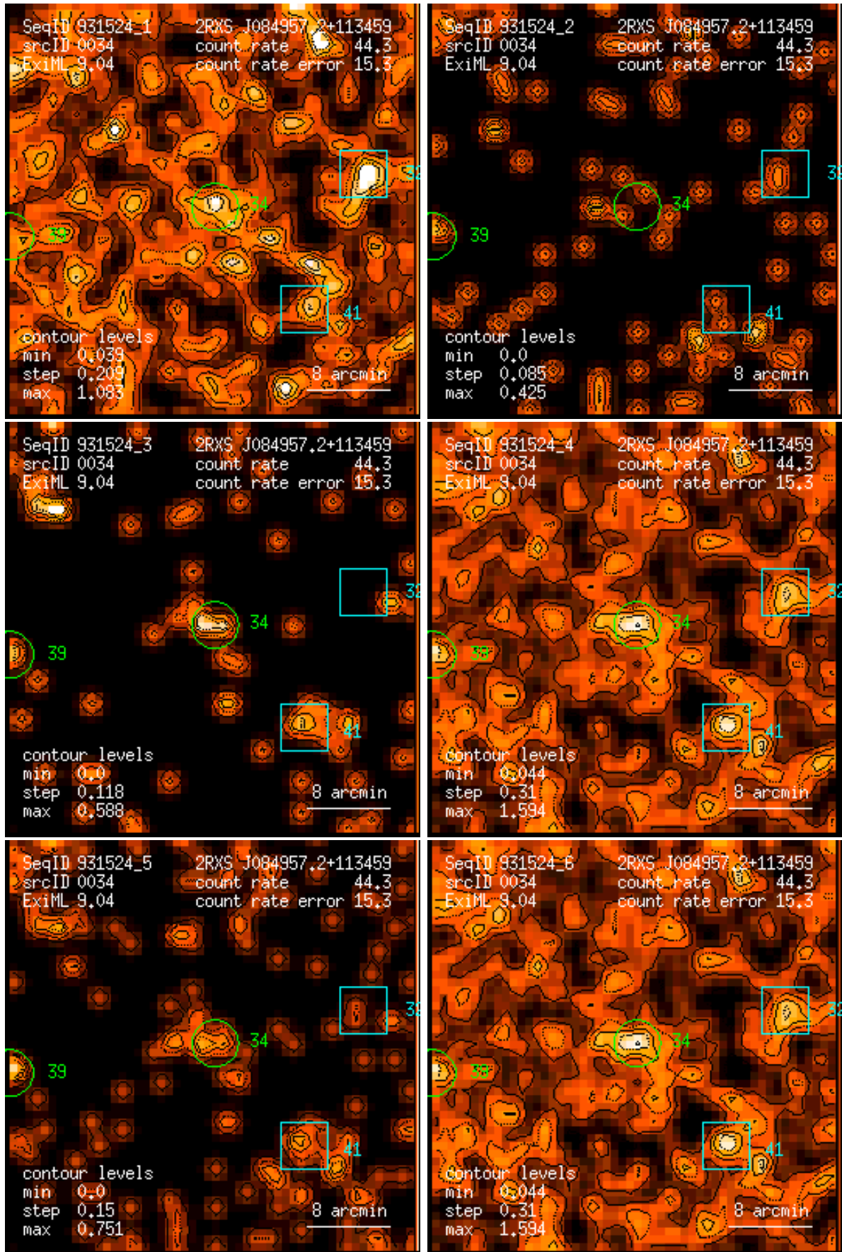
Figure 34: RASS 931524: detection 0034: band rate images, Gaussian filter: (1) PSPC channels 11 – 41, (2) 52 – 90, (3) 91 – 201, (4) 11 – 235, (5) 52 – 201, (6) 11 – 201. Broad band rates in counts/ks. Band rate contour levels in counts/ks/arcmin 2 .
