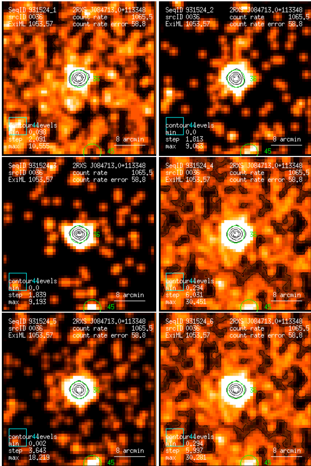
Figure 36: RASS 931524: detection 0036: band rate images, Gaussian filter: (1) PSPC channels 11 – 41, (2) 52 – 90, (3) 91 – 201, (4) 11 – 235, (5) 52 – 201, (6) 11 – 201. Broad band rates in counts/ks. Band rate contour levels in counts/ks/arcmin 2 .
