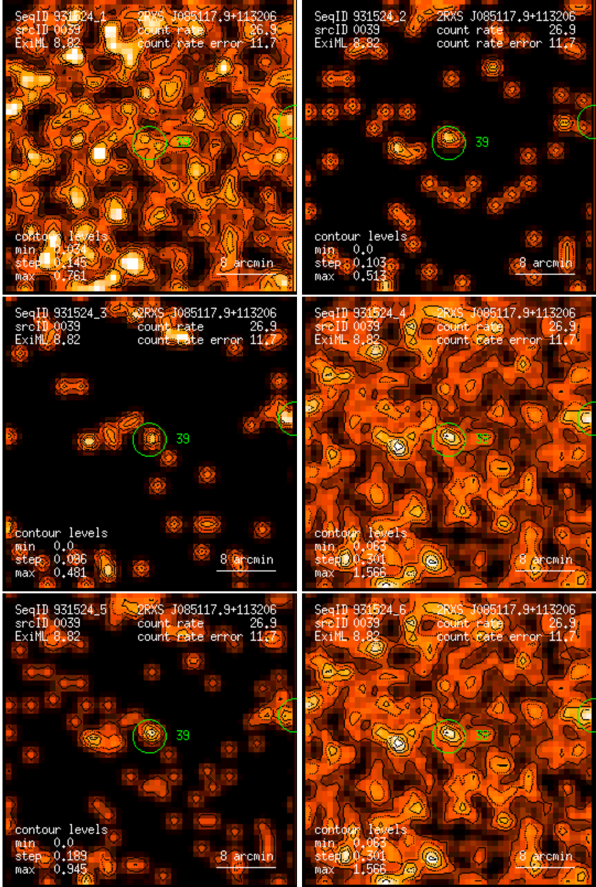
Figure 39: RASS 931524: detection 0039: band rate images, Gaussian filter: (1) PSPC channels 11 – 41, (2) 52 – 90, (3) 91 – 201, (4) 11 – 235, (5) 52 – 201, (6) 11 – 201. Broad band rates in counts/ks. Band rate contour levels in counts/ks/arcmin 2 .
