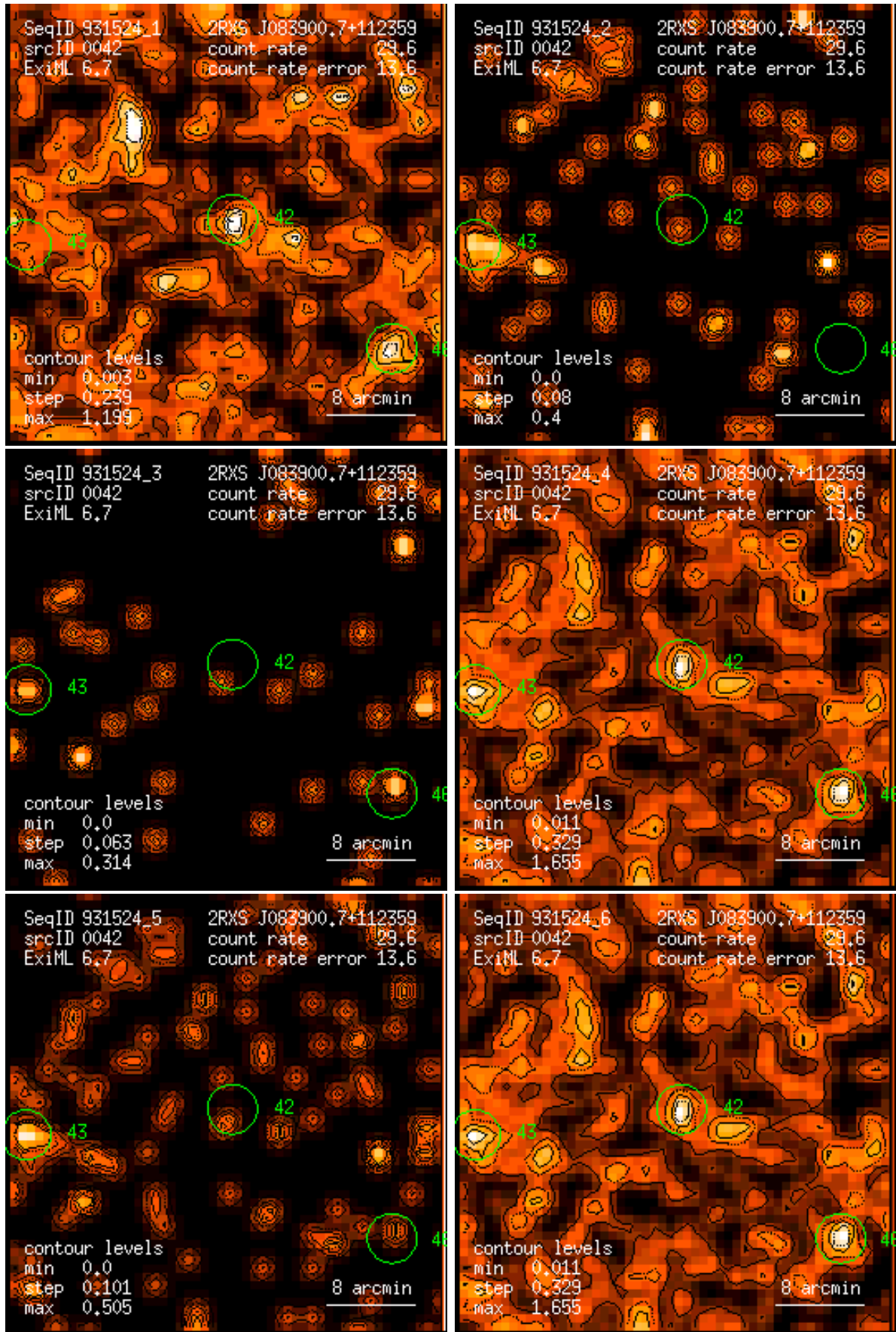
Figure 42: RASS 931524: detection 0042: band rate images, Gaussian filter: (1) PSPC channels 11 – 41, (2) 52 – 90, (3) 91 – 201, (4) 11 – 235, (5) 52 – 201, (6) 11 – 201. Broad band rates in counts/ks. Band rate contour levels in counts/ks/arcmin 2 .
