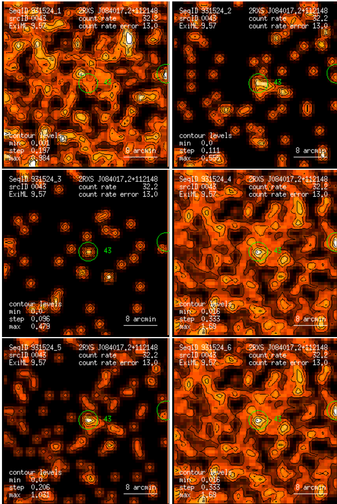
Figure 43: RASS 931524: detection 0043: band rate images, Gaussian filter: (1) PSPC channels 11 – 41, (2) 52 – 90, (3) 91 – 201, (4) 11 – 235, (5) 52 – 201, (6) 11 – 201. Broad band rates in counts/ks. Band rate contour levels in counts/ks/arcmin 2 .
