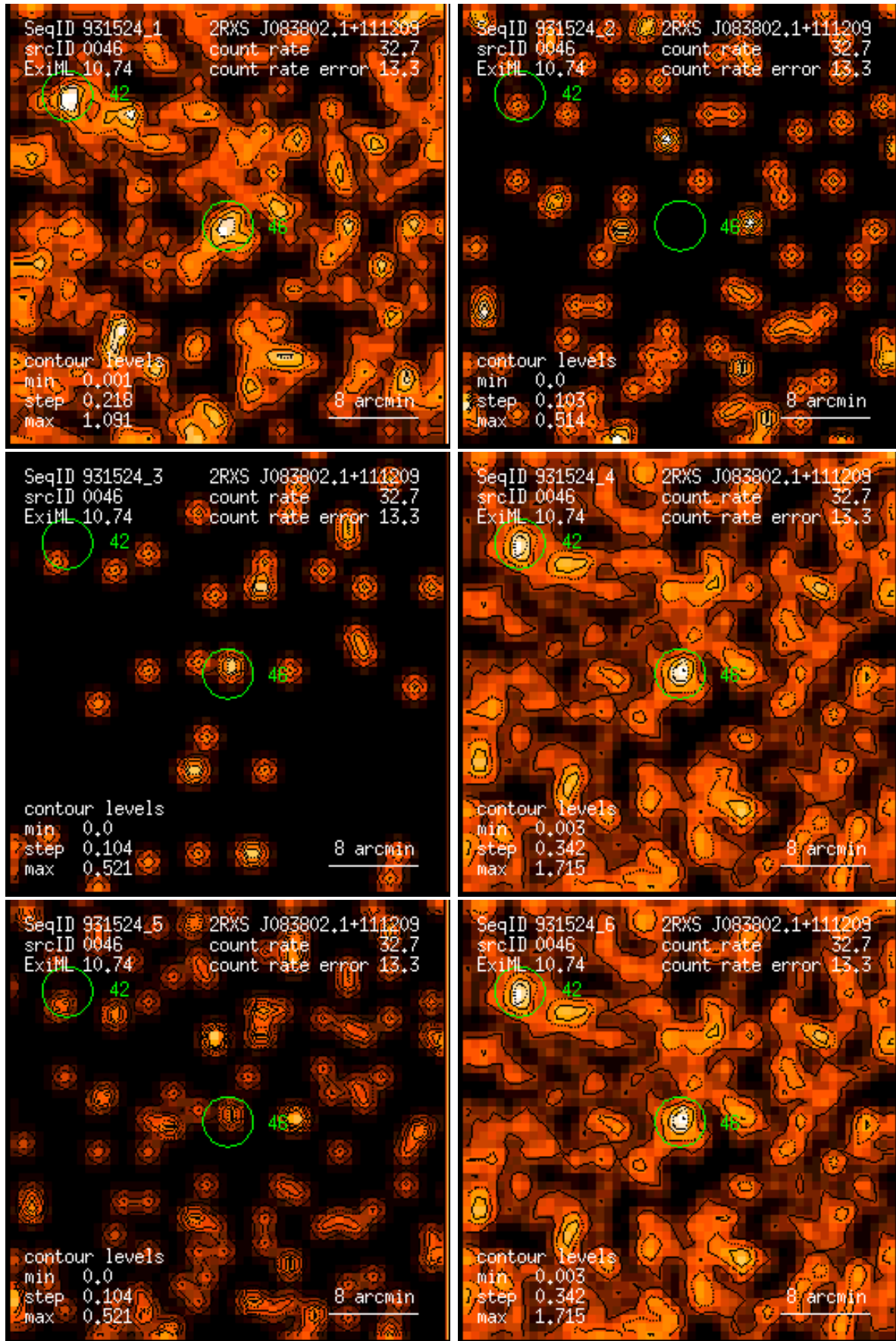
Figure 46: RASS 931524: detection 0046: band rate images, Gaussian filter: (1) PSPC channels 11 – 41, (2) 52 – 90, (3) 91 – 201, (4) 11 – 235, (5) 52 – 201, (6) 11 – 201. Broad band rates in counts/ks. Band rate contour levels in counts/ks/arcmin 2 .
