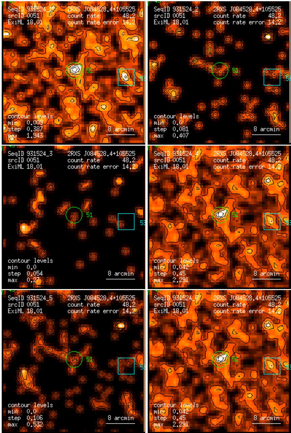
Figure 51: RASS 931524: detection 0051: band rate images, Gaussian filter: (1) PSPC channels 11 – 41, (2) 52 – 90, (3) 91 – 201, (4) 11 – 235, (5) 52 – 201, (6) 11 – 201. Broad band rates in counts/ks. Band rate contour levels in counts/ks/arcmin 2 .
