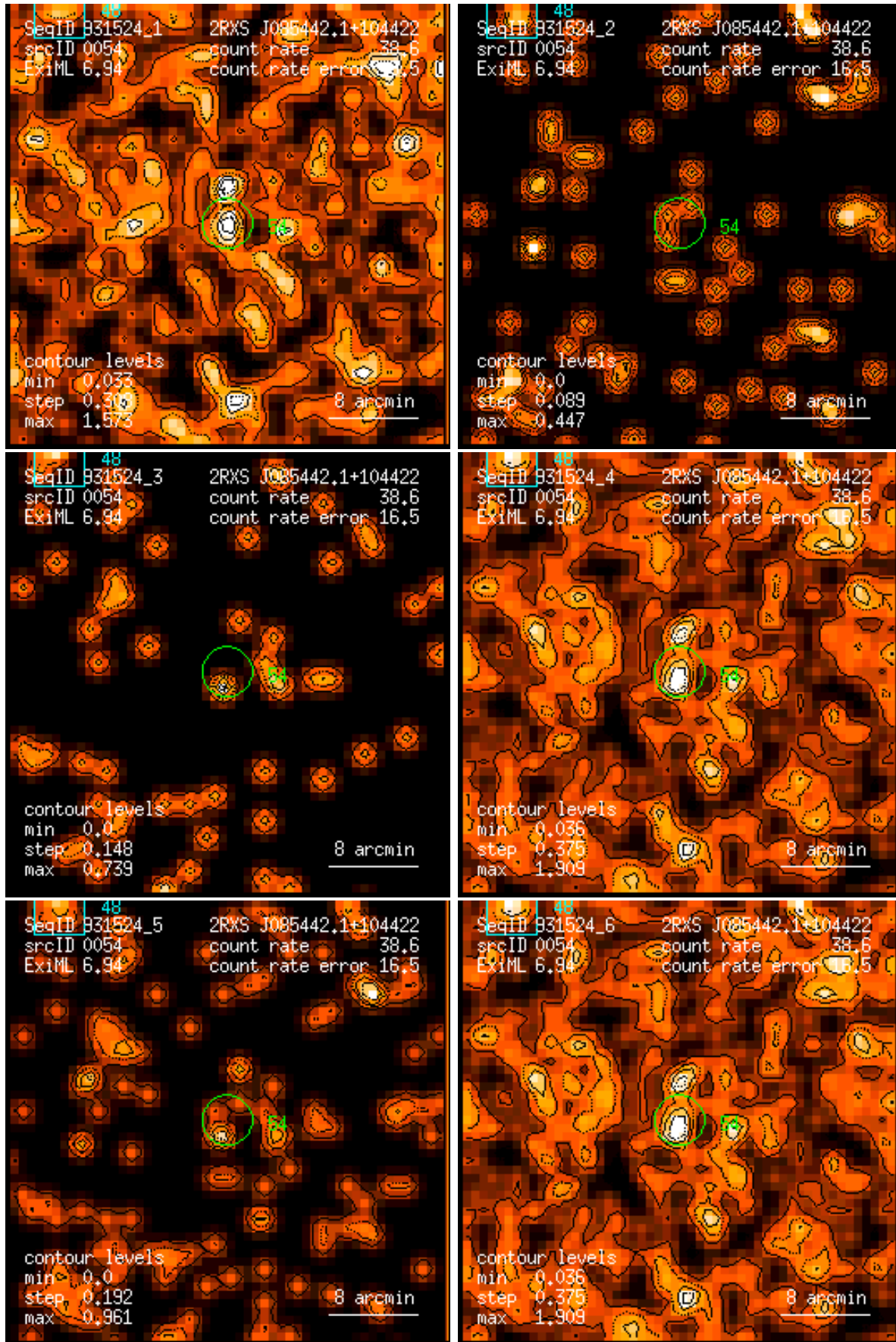
Figure 54: RASS 931524: detection 0054: band rate images, Gaussian filter: (1) PSPC channels 11 – 41, (2) 52 – 90, (3) 91 – 201, (4) 11 – 235, (5) 52 – 201, (6) 11 – 201. Broad band rates in counts/ks. Band rate contour levels in counts/ks/arcmin 2 .
