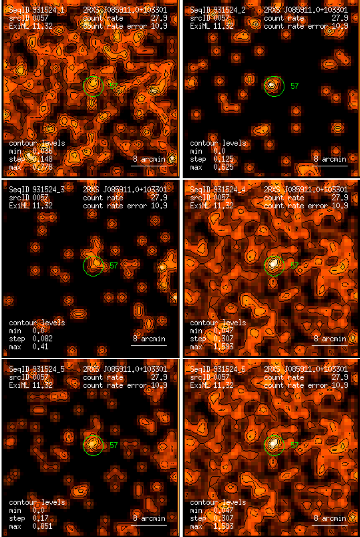
Figure 57: RASS 931524: detection 0057: band rate images, Gaussian filter: (1) PSPC channels 11 – 41, (2) 52 – 90, (3) 91 – 201, (4) 11 – 235, (5) 52 – 201, (6) 11 – 201. Broad band rates in counts/ks. Band rate contour levels in counts/ks/arcmin 2 .
