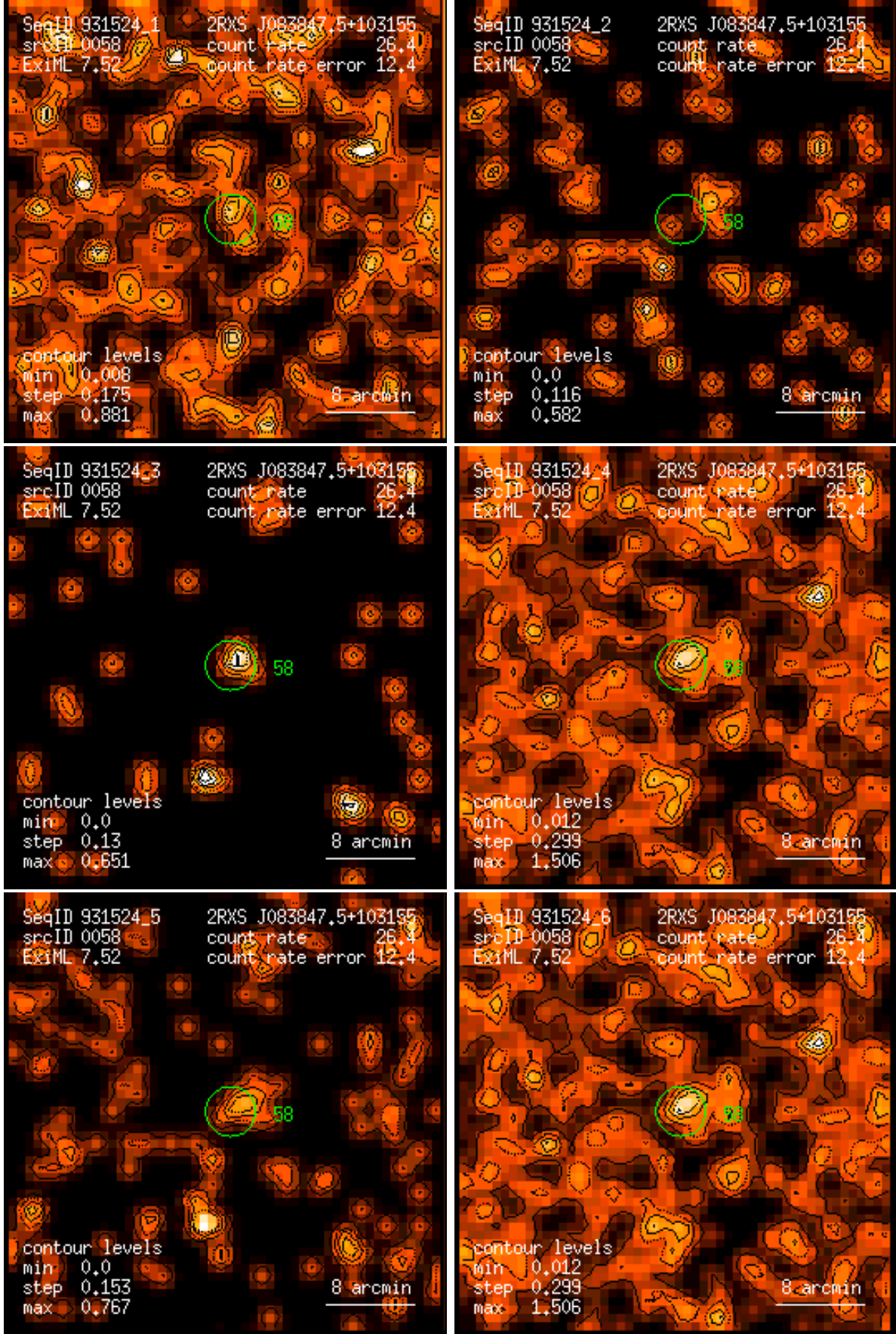
Figure 58: RASS 931524: detection 0058: band rate images, Gaussian filter: (1) PSPC channels 11 – 41, (2) 52 – 90, (3) 91 – 201, (4) 11 – 235, (5) 52 – 201, (6) 11 – 201. Broad band rates in counts/ks. Band rate contour levels in counts/ks/arcmin 2 .
