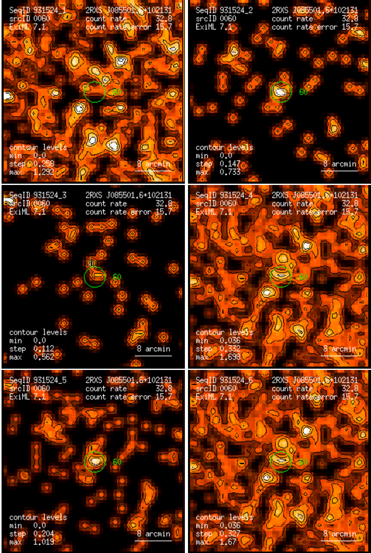
Figure 60: RASS 931524: detection 0060: band rate images, Gaussian filter: (1) PSPC channels 11 – 41, (2) 52 – 90, (3) 91 – 201, (4) 11 – 235, (5) 52 – 201, (6) 11 – 201. Broad band rates in counts/ks. Band rate contour levels in counts/ks/arcmin 2 .
