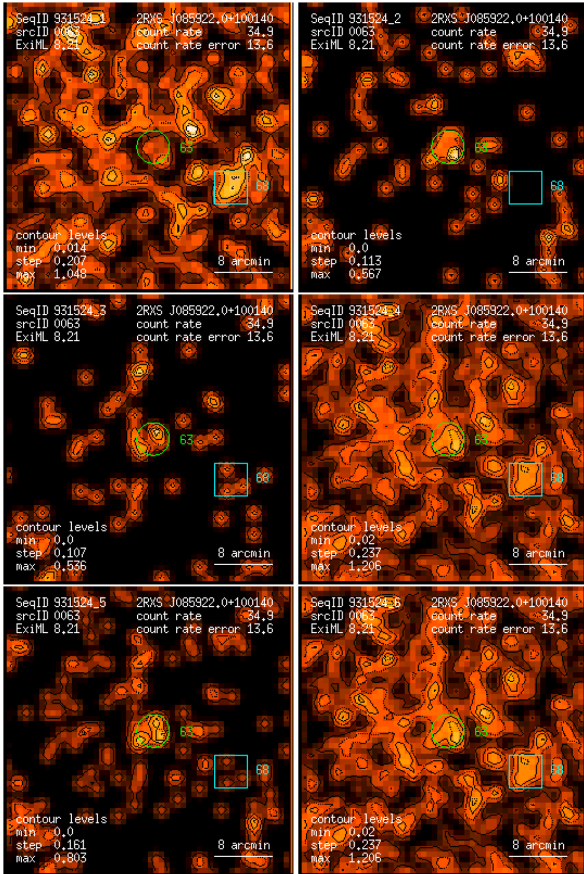
Figure 63: RASS 931524: detection 0063: band rate images, Gaussian filter: (1) PSPC channels 11 – 41, (2) 52 – 90, (3) 91 – 201, (4) 11 – 235, (5) 52 – 201, (6) 11 – 201. Broad band rates in counts/ks. Band rate contour levels in counts/ks/arcmin 2 .
