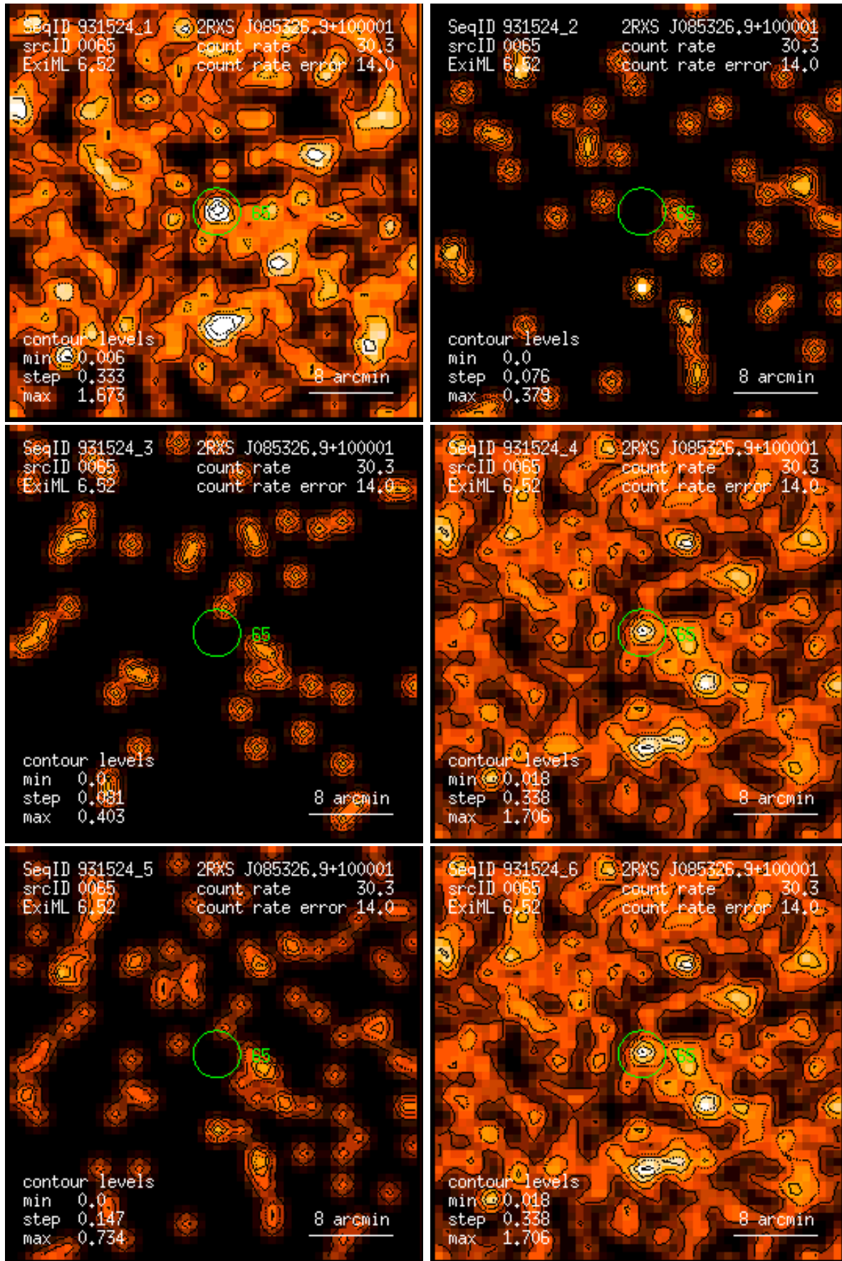
Figure 65: RASS 931524: detection 0065: band rate images, Gaussian filter: (1) PSPC channels 11 – 41, (2) 52 – 90, (3) 91 – 201, (4) 11 – 235, (5) 52 – 201, (6) 11 – 201. Broad band rates in counts/ks. Band rate contour levels in counts/ks/arcmin 2 .
